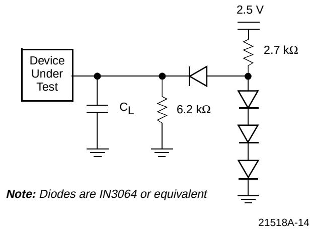
Figure 12. Test Setup
