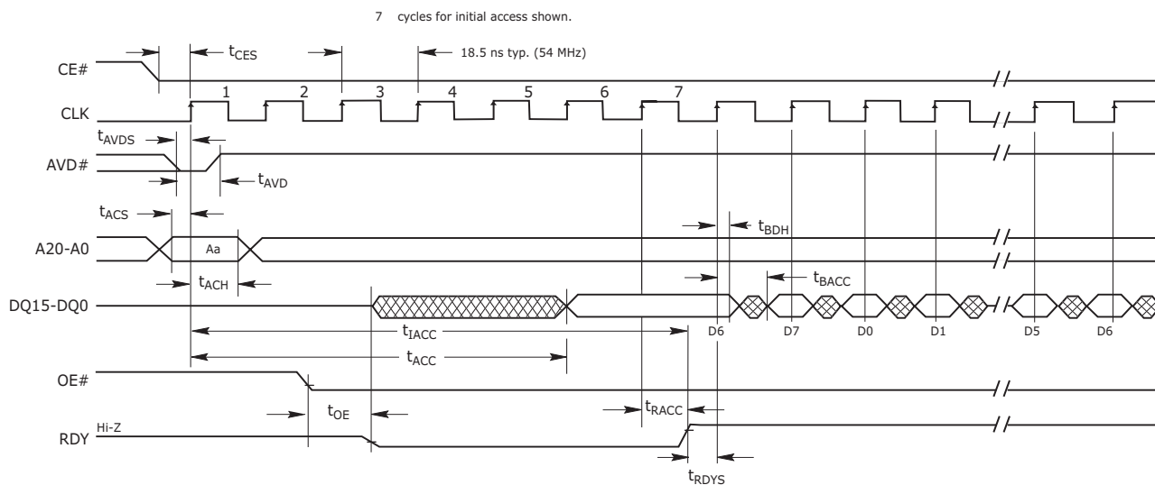
Figure I3. Synchronous Burst Mode Read
