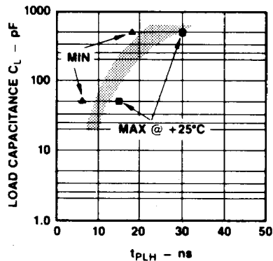
Figure 5. t_{PLH} for V_{OH} = 2.7\text{ Vol} vs. C_L .
