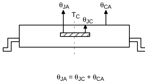
Figure 13. Thermal Resistance — °C/Watt
