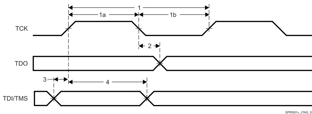
Figure 6-23. JTAG Timing
