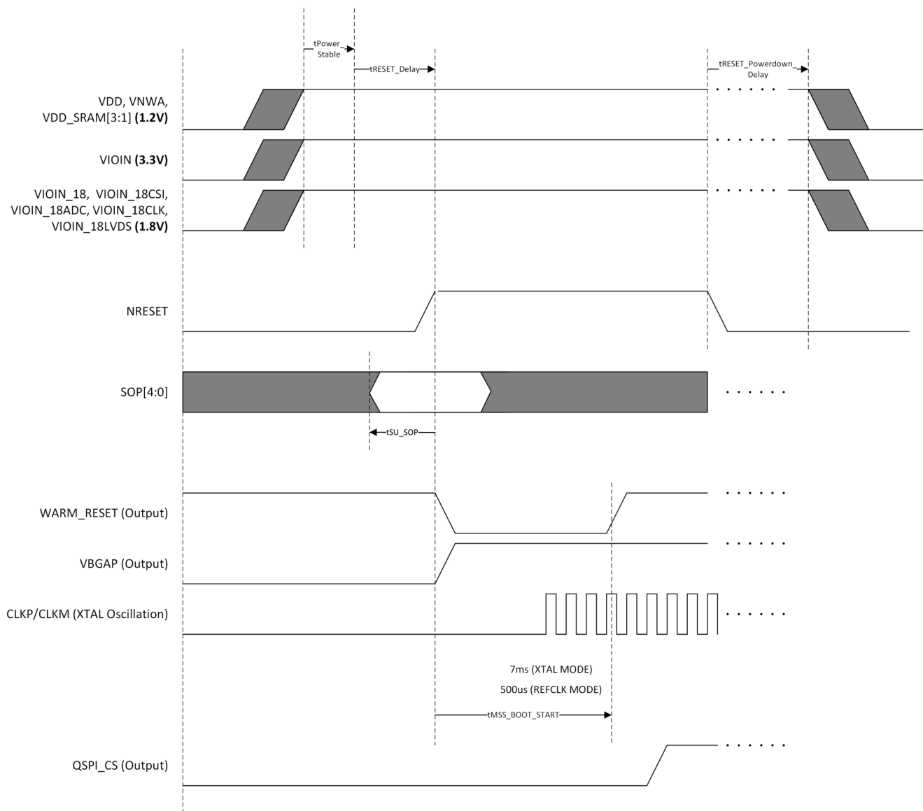
Figure 6-1. Device Wake-up and Power-Down Sequence
