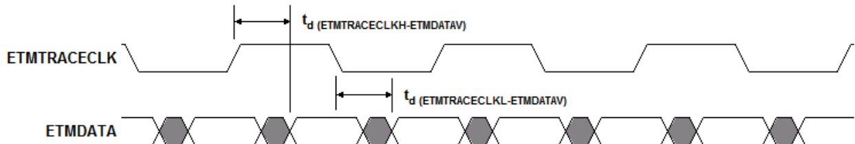
Figure 6-25. ETMDATA Timing
