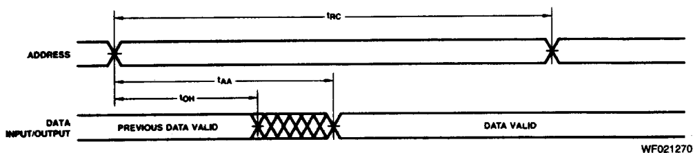
Read Cycle No. 1 ( \overline{WE} HIGH, \overline{CE} LOW)
