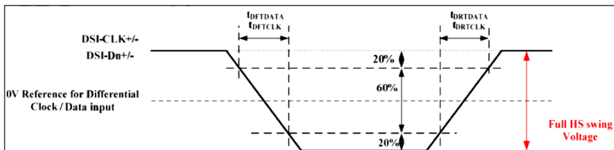
AC characteristics for MIPI-DSI High speed mode
