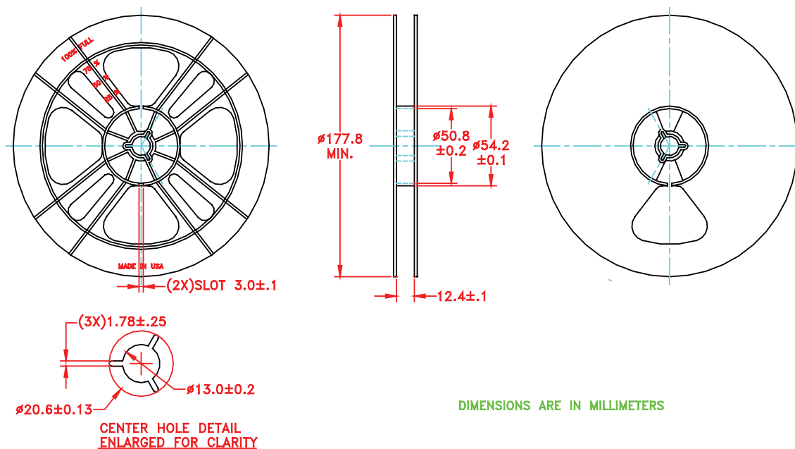
Figure 13: Carrier Tape
