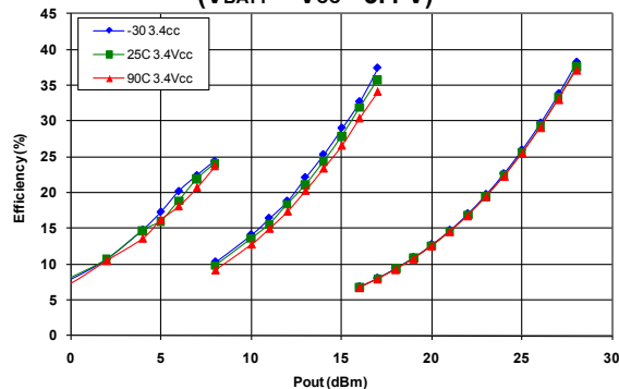
Figure 5: LTE PAE (%) over Temperature ( V_{BATT} = V_{CC} = 3.4 V)
