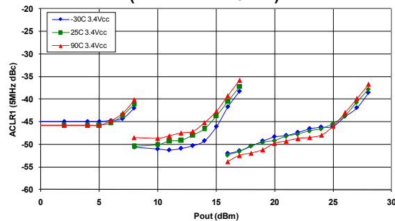
Figure 7: LTE ACLR1 (dBc) over Temperature ( V_{BATT} = V_{CC} = 3.4 V)
