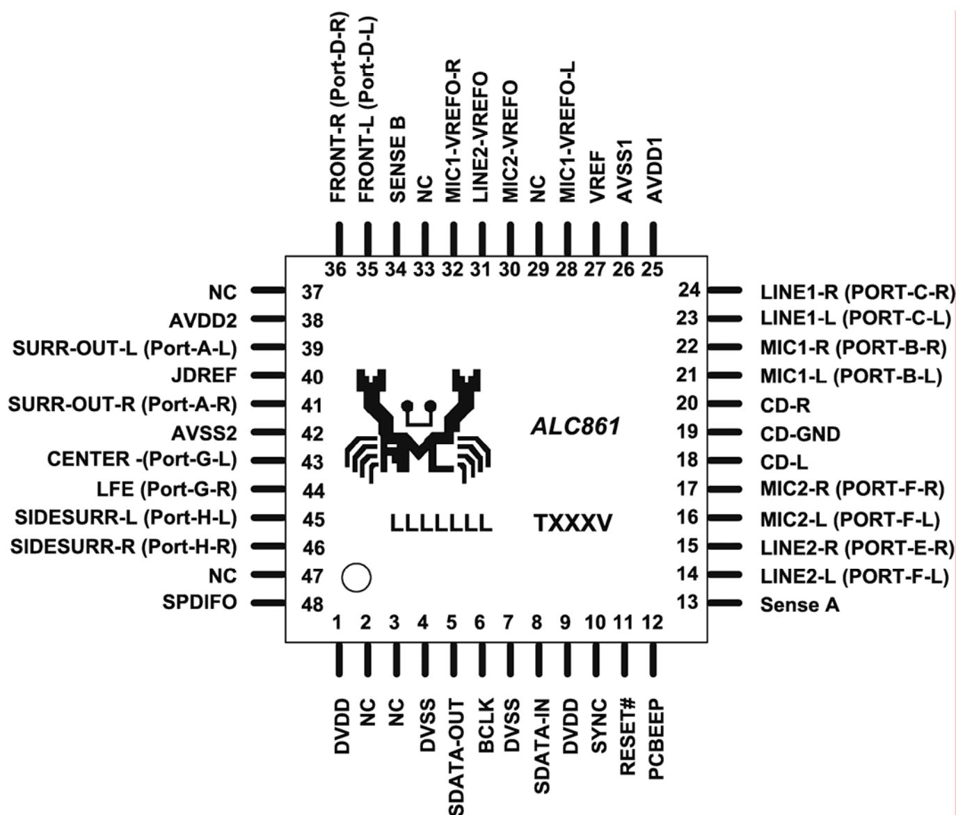
Figure 2. Pin Assignments
