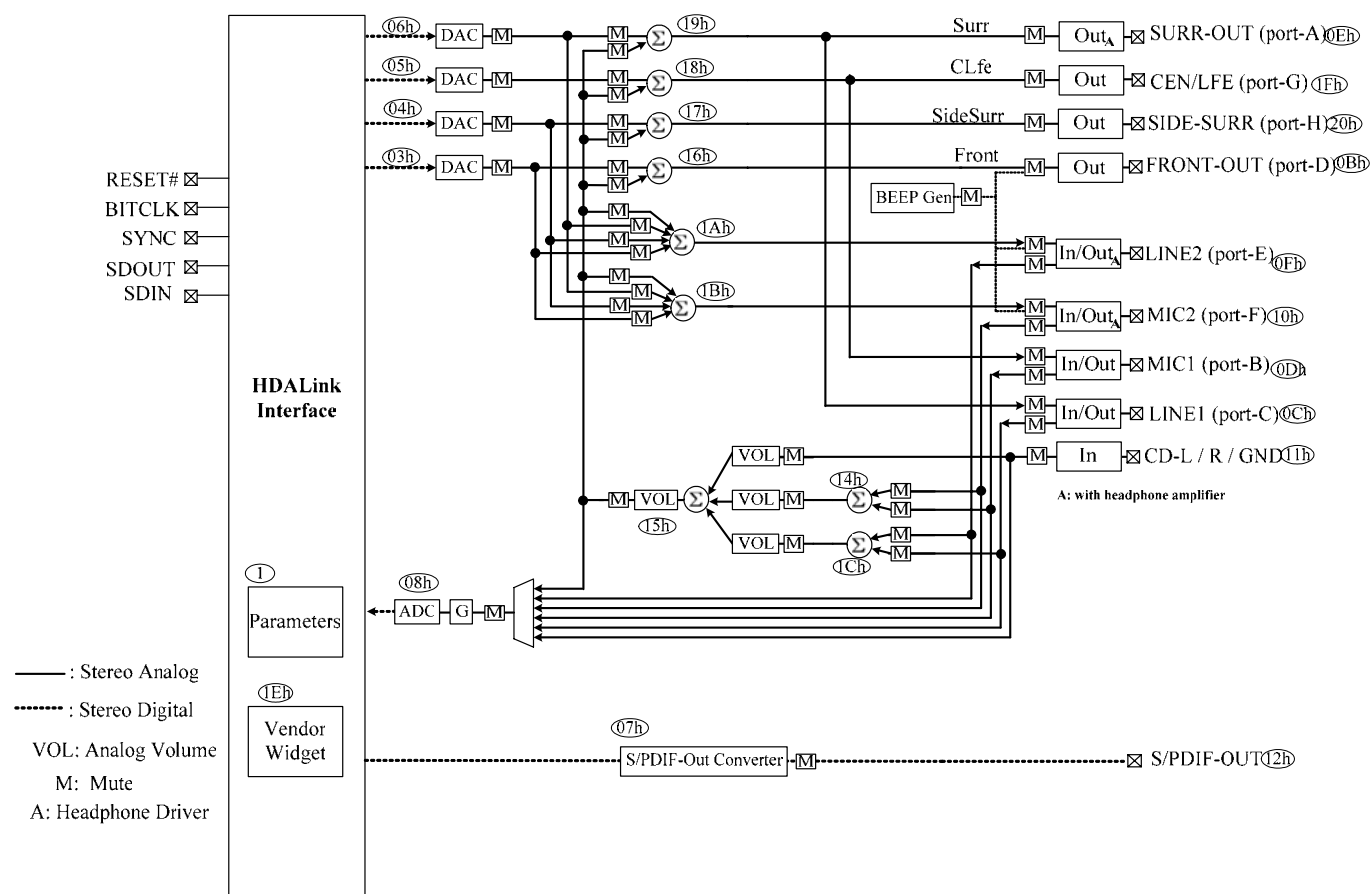
Figure 1. Block Diagram
