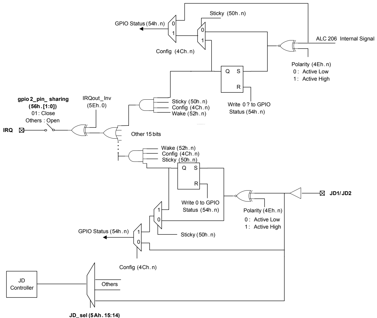
Figure 19. Jack Detect and IRQ Logic
