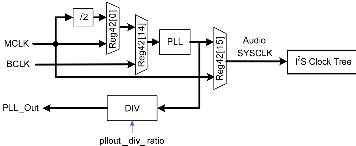
Figure 4. Audio SYSCLK
