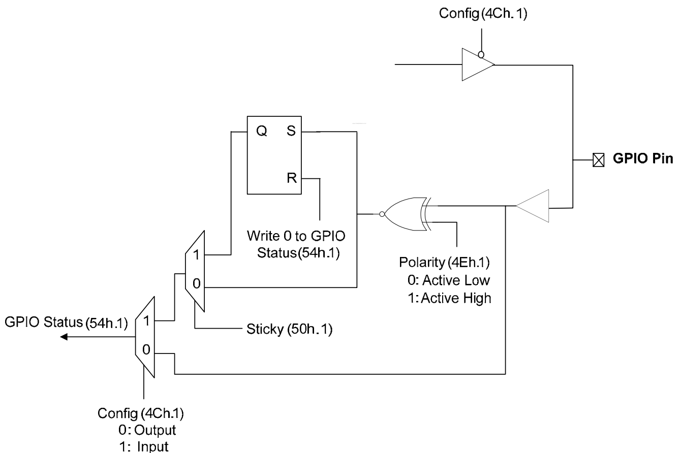
Figure 18. GPIO Implementation
