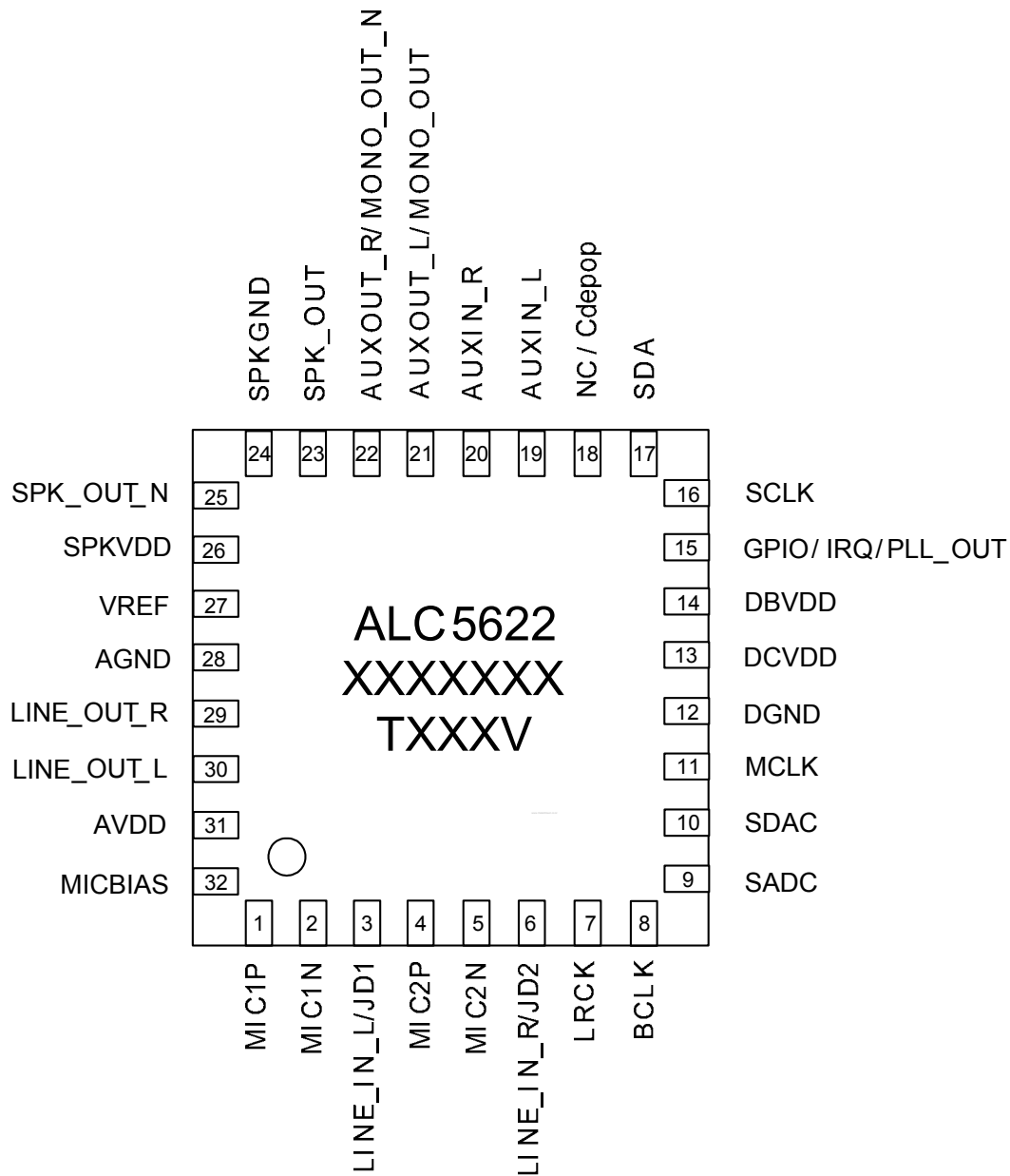
Figure 3. Pin Assignments
