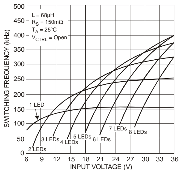
Figure 22 Switching Frequency vs. Input Voltage
