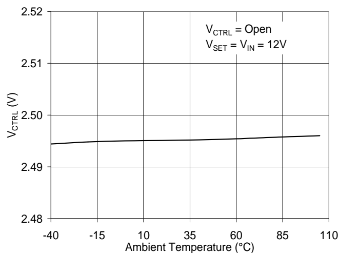
Figure 4 V_{CTRL} vs. Temperature
