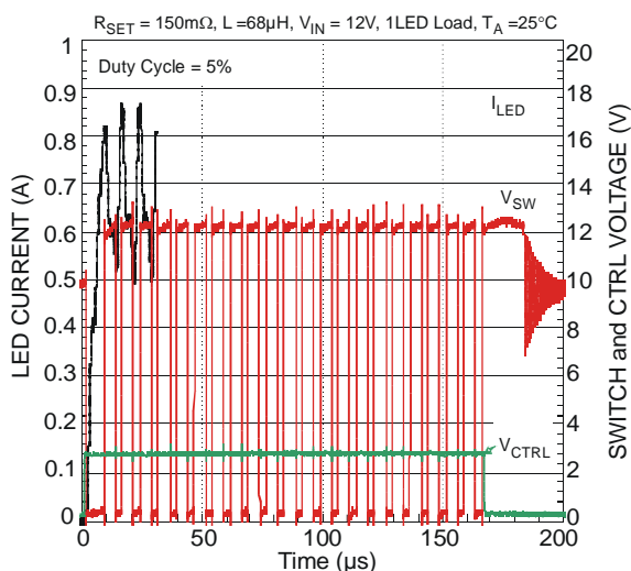
Figure 11 PWM Dimming
