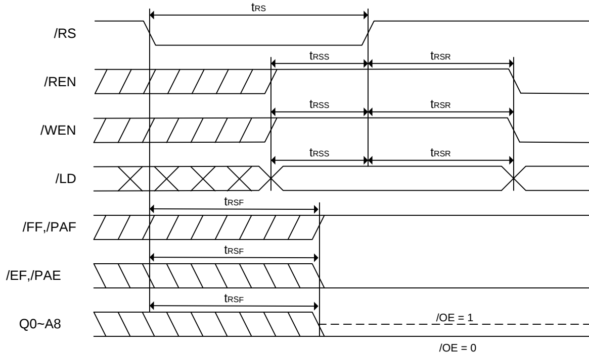
Figure 3. Reset Timing
