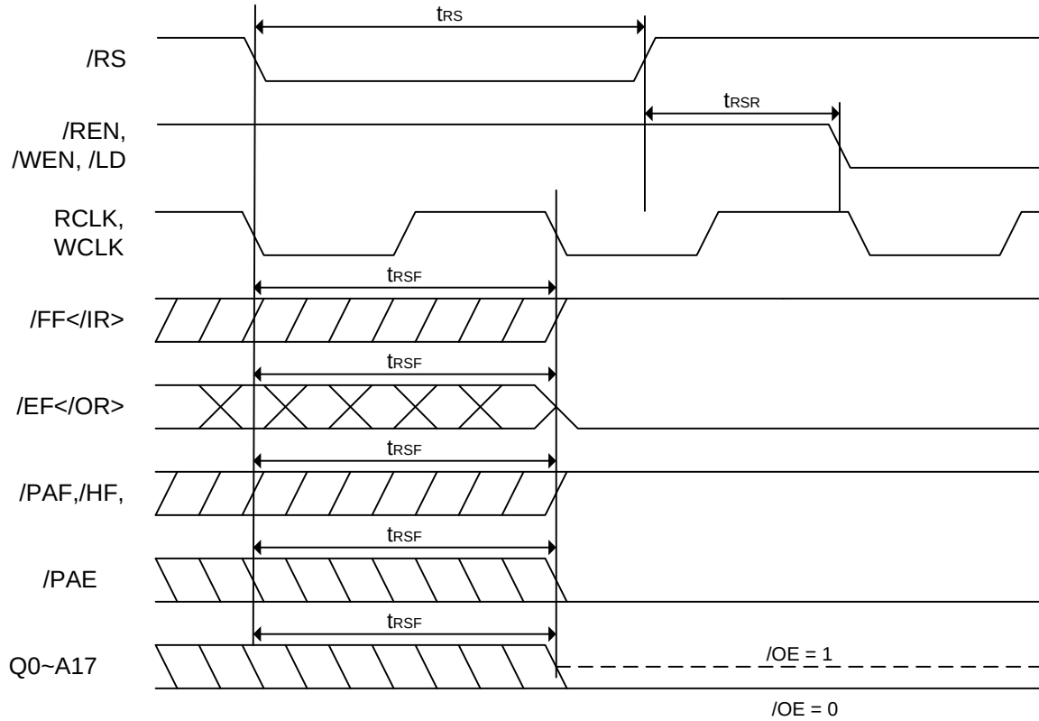
Figure 2. Reset Timing
