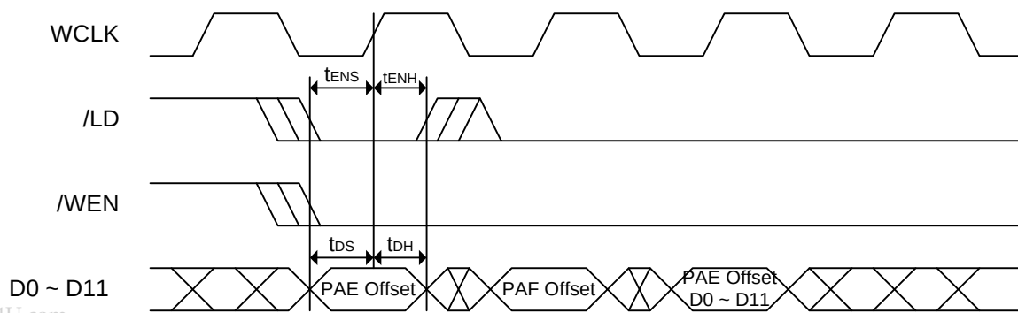
Figure 3. Write Programmable Registers
