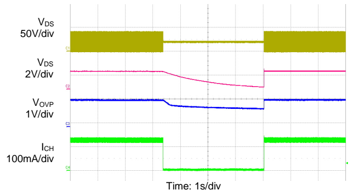
Overtemperature Protection
