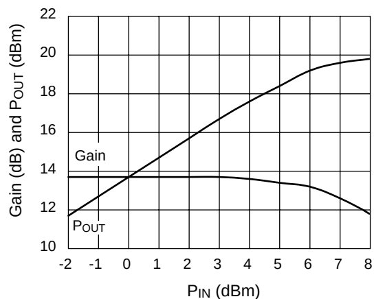
P OUT and Gain vs. P IN 900 MHz
