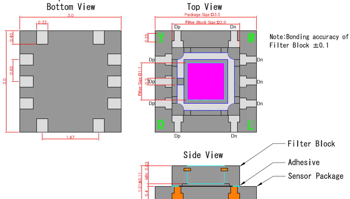
Figure 12.1 Outline Dimensions
