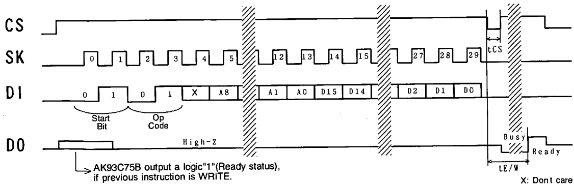
WRITE (AK93C75B)
