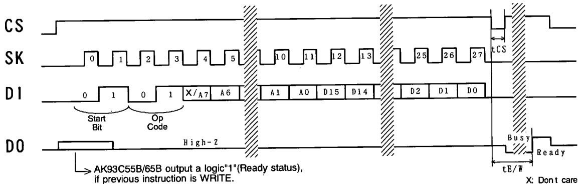
WRITE (AK93C55B/65B)
