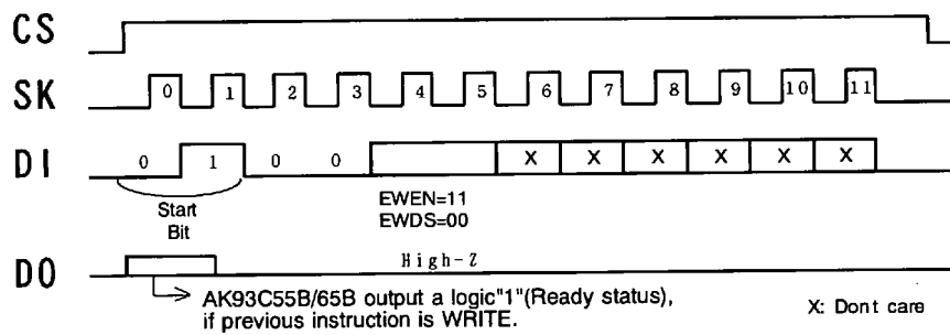
EWEN/EWDS (AK93C55B/65B)
