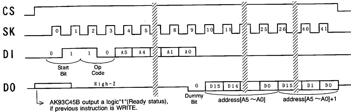
READ (AK93C45B)
