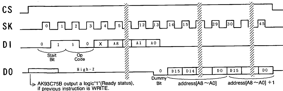
READ (AK93C75B)
