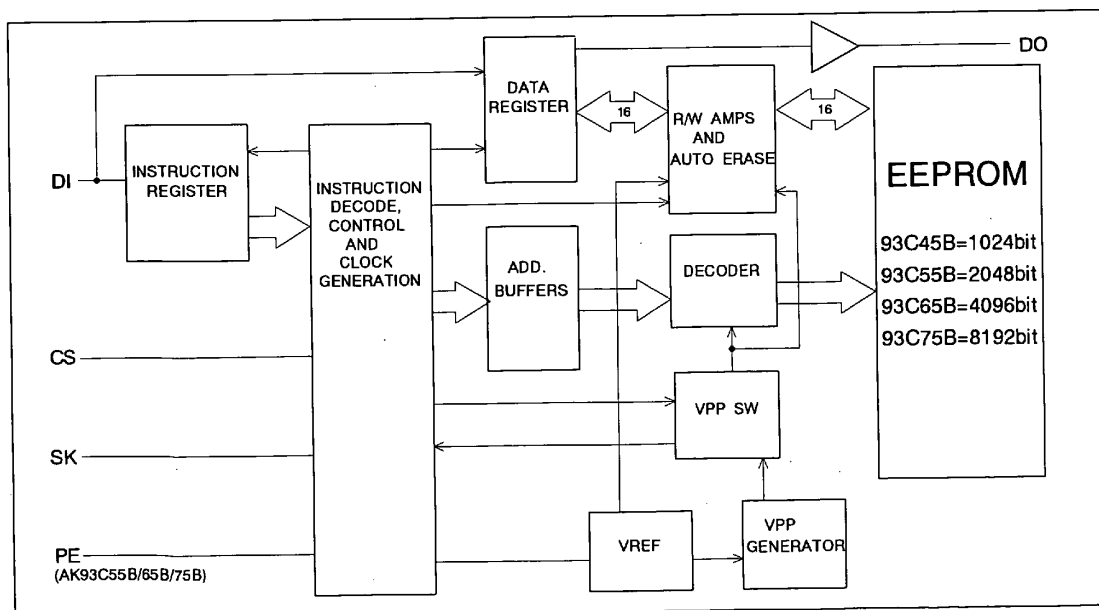
Block Diagram
