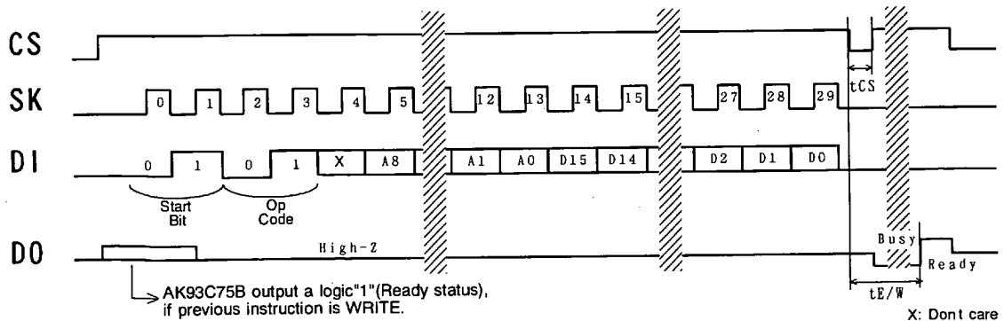
WRITE (AK93C75B)
