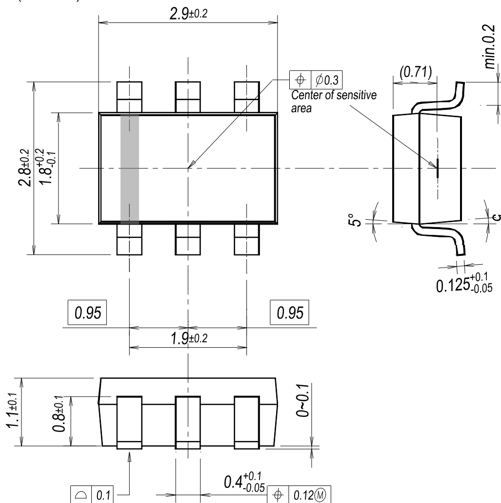
Figure 12. Outline Dimensions
