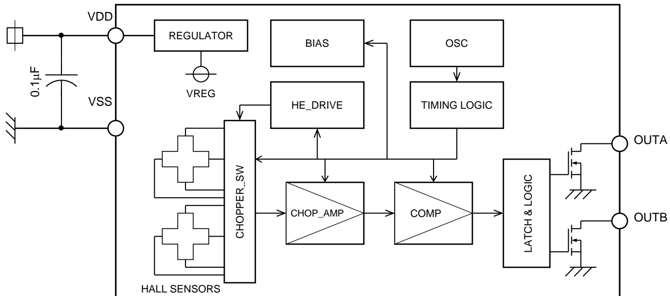
Figure 1. AK8779B Block Diagram
