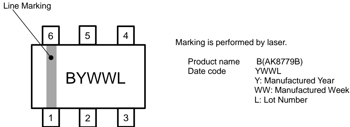
Figure 14. Marking
