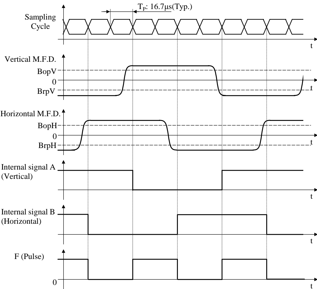
Figure 5. Timing diagram
