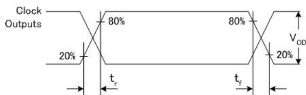
Figure 4 Output Rise/Fall Time
