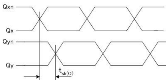
Figure 3 Output Skew
