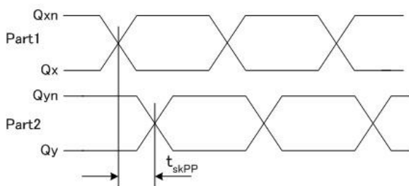
Figure 7 Part-to-Part Skew
