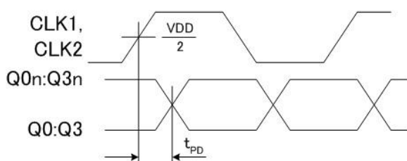
Figure 5 Propagation Delay
