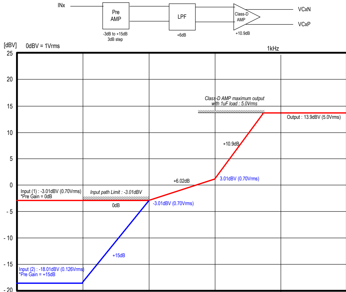
Figure 14. Level Diagram
