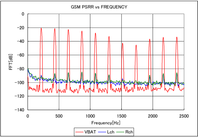
Figure 13. “GSM PSRR vs TIME” & “GSM PSRR vs Frequency”
