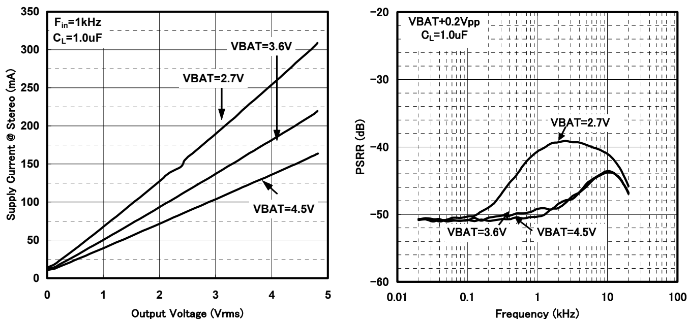
Figure 10. " Supply Current vs. Output Voltage " &amp; " Supply Ripple Rejection Ratio vs Frequency "
