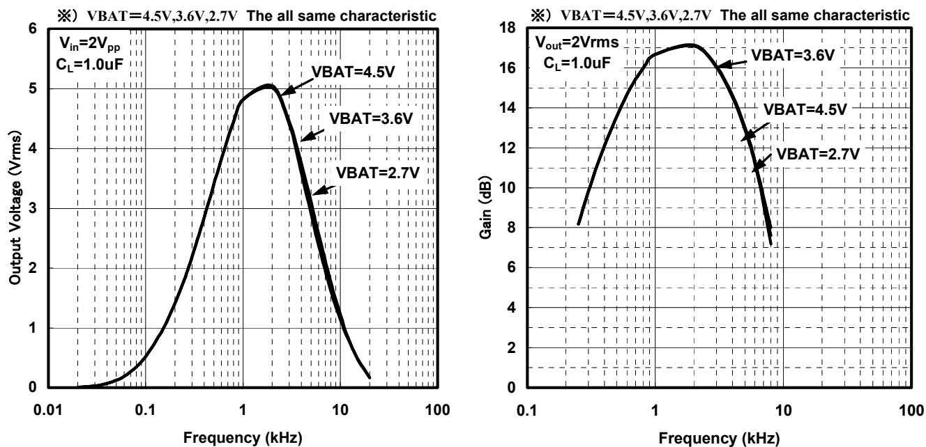
Figure 9. " Output Amplitude vs. Frequency " &amp; " Frequency Response "
