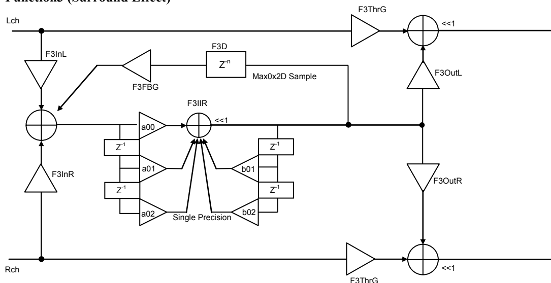
Figure 35. Function3 Block Diagram
