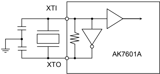
Figure 9. X'tal Mode
