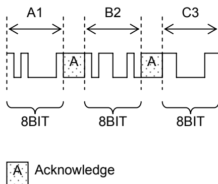
Figure 27. Division of the Data
