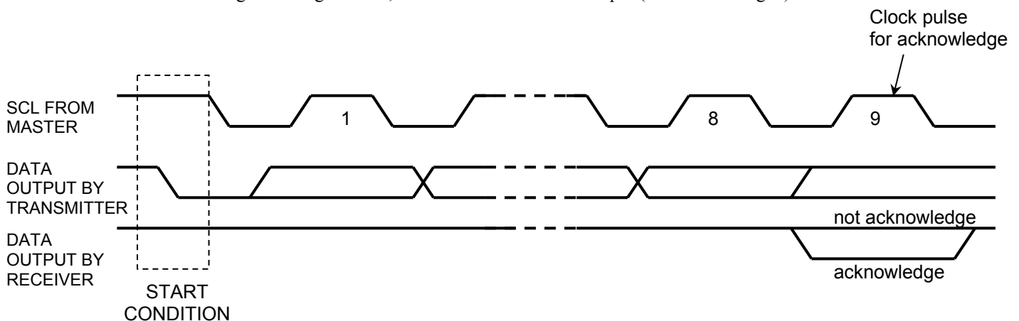
Figure 25. Acknowledge
