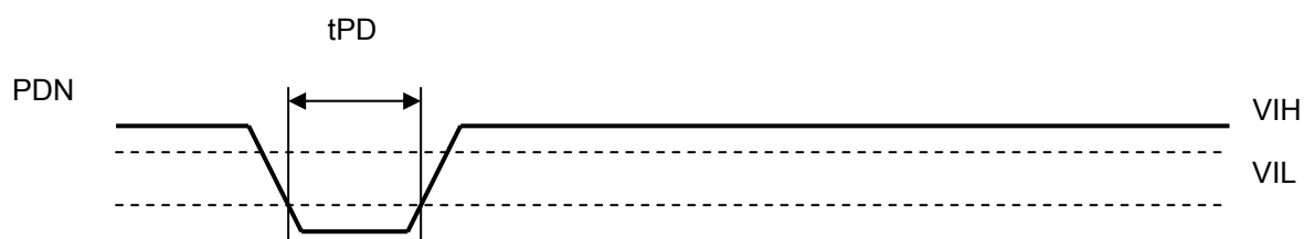
Figure 7. Power Down &amp; Reset Timing
