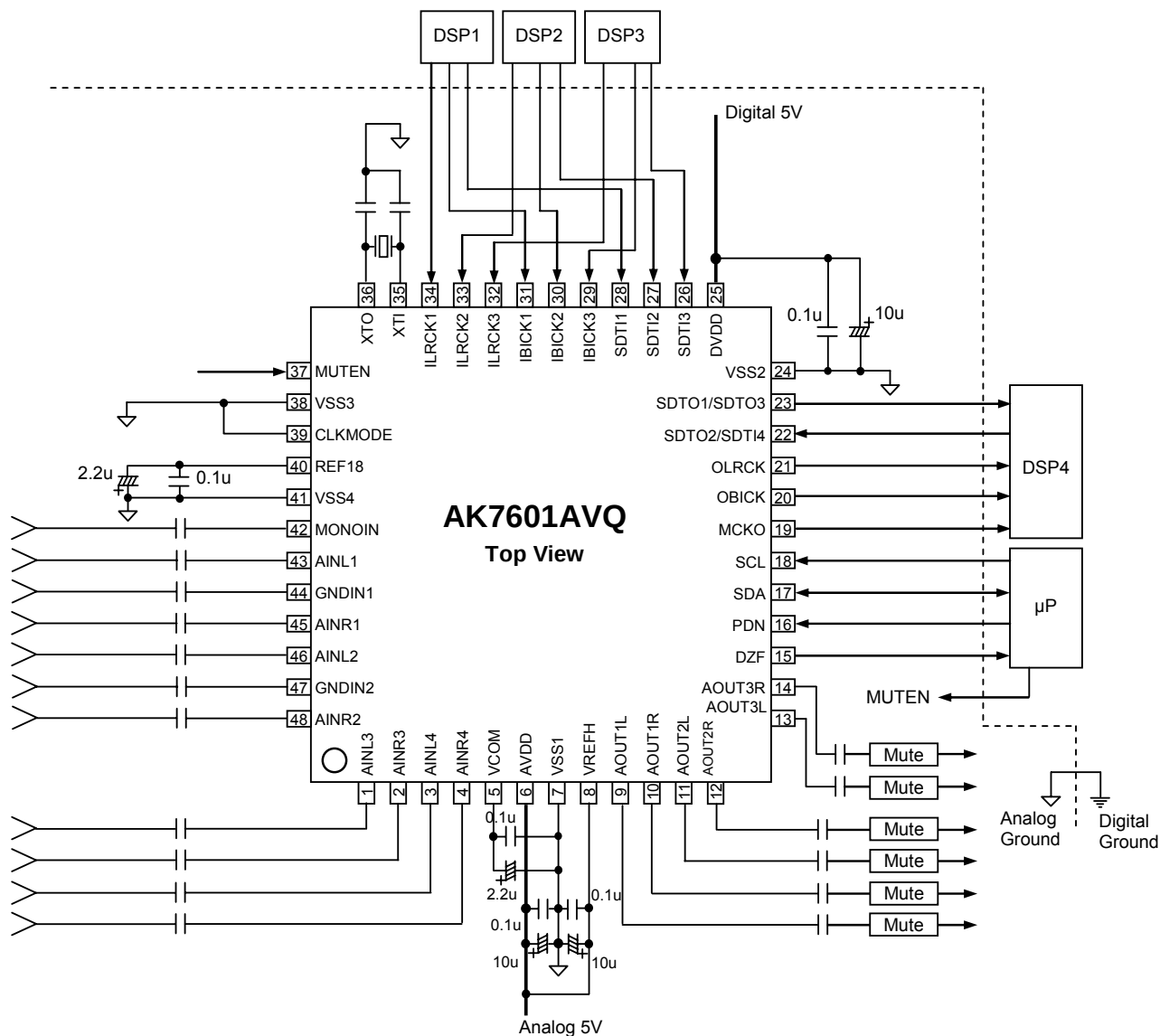
Figure 42. System Connection Diagram
