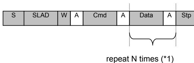
Figure 28. Write Sequence
