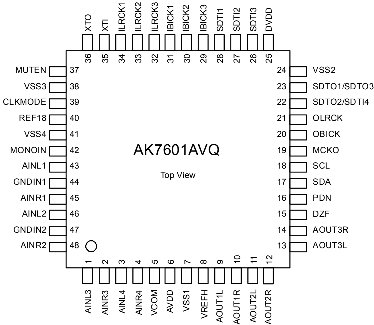
Figure 2. Pin Layout
