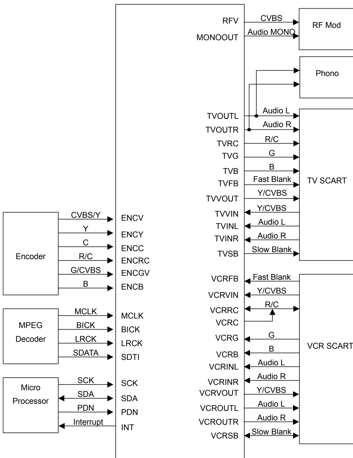
Figure 19. Typical Connection Diagram
