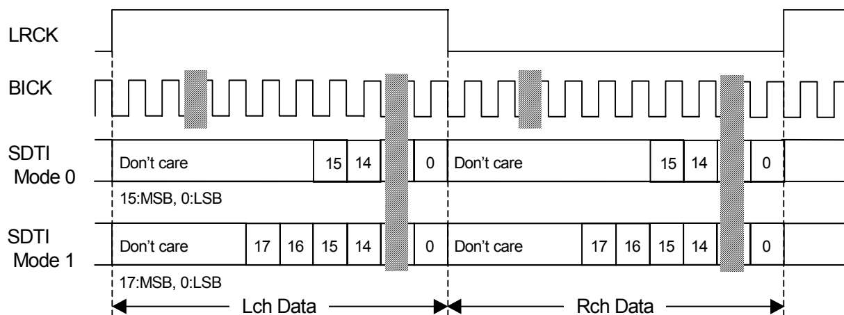
Figure 4. Mode 0,1 Timing
