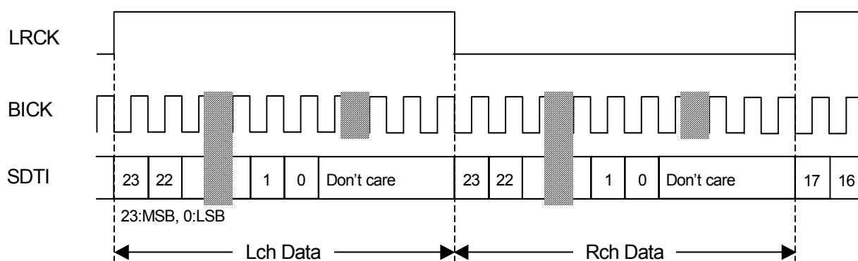
Figure 5. Mode 2 Timing
