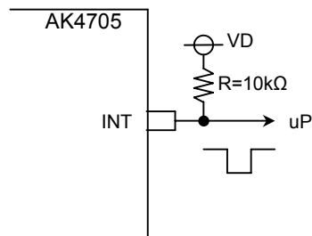
Figure 9. INT pin
