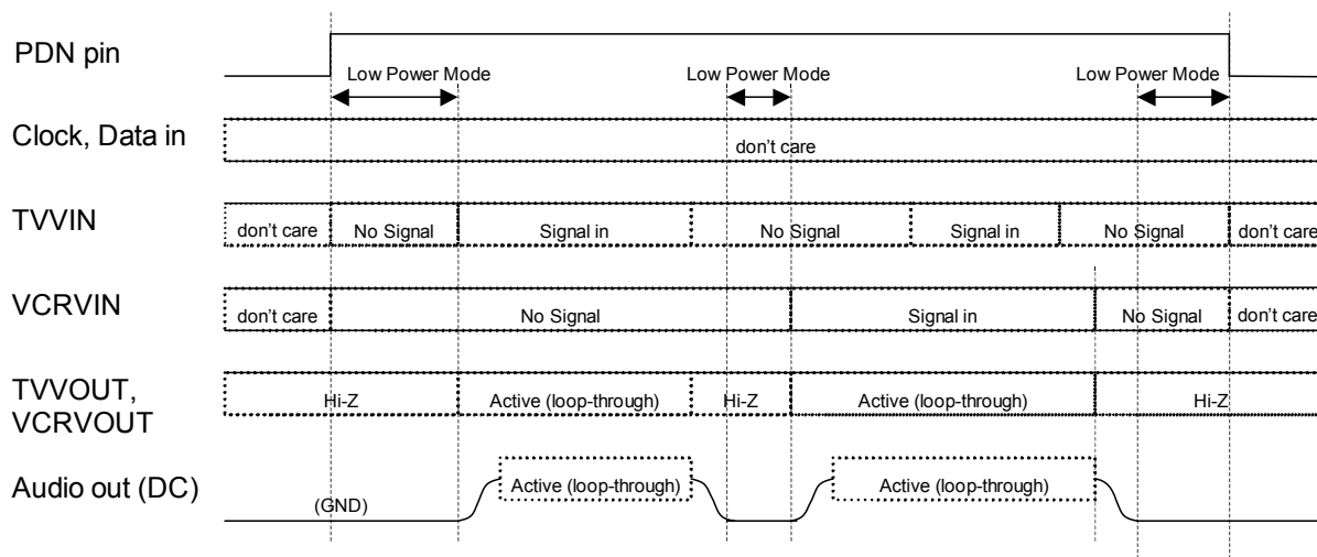
Figure 2. Typical operating sequence (auto setup mode)
