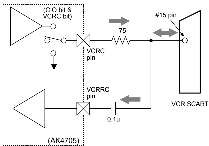
Figure 8. Red/Chroma Bi-directional Control
