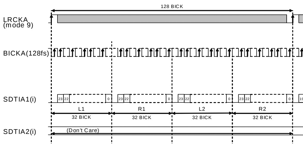
Figure 6. Mode 9 Timing
