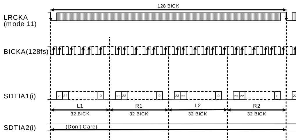
Figure 8. Mode 11 Timing
