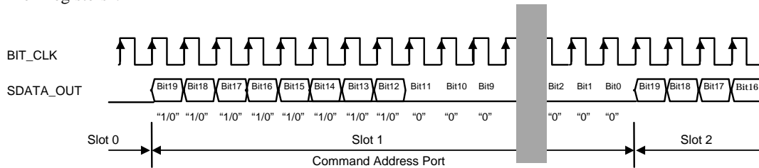
Figure 36. Slot 1
