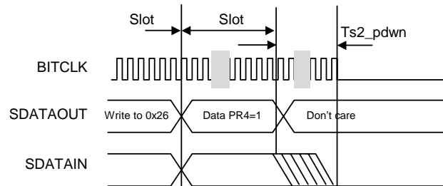
Figure 9. AC-link Low Power Mode Timing
