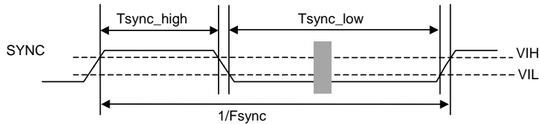
Figure 4. SYNC Timing
