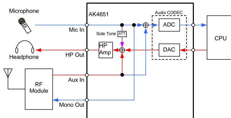
Figure 32. Recording/Playback &amp; Phone
