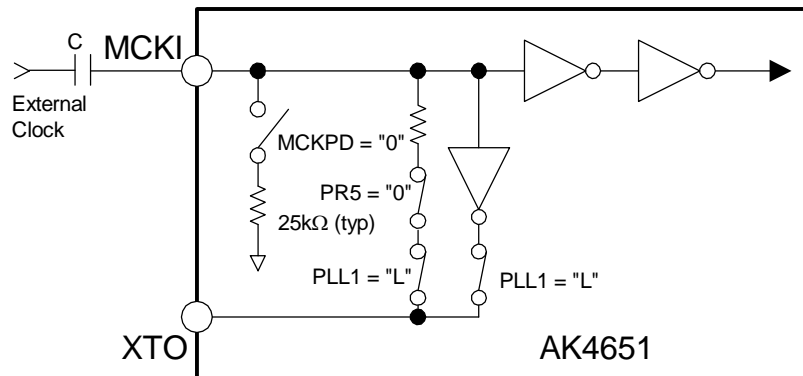
Figure 14. External Clock mode (Input : \geq 50\%DVDD ) Note 36. This clock level must not exceed DVDD level. (C : 0.1μF)
