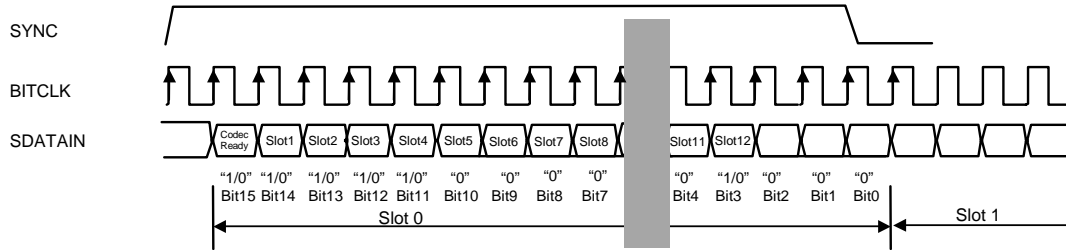
Figure 38. Slot 0
