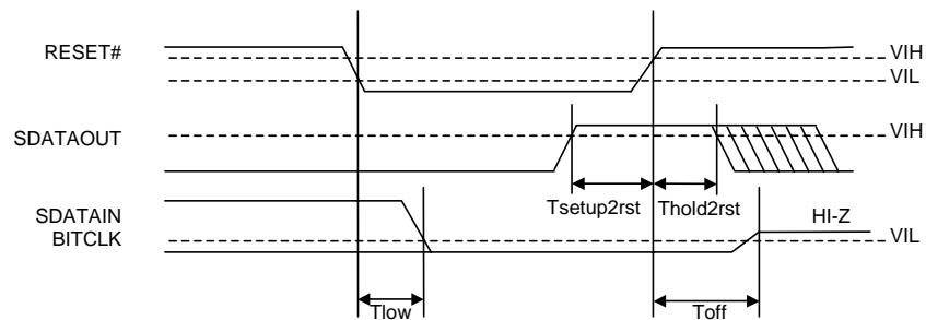
Figure 10. Activate Test Mode Timing
