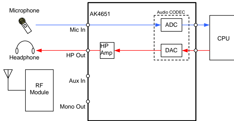
Figure 30. MIC recording &amp; Headphone playback
