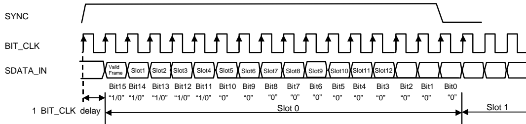
Figure 35. Slot 0
