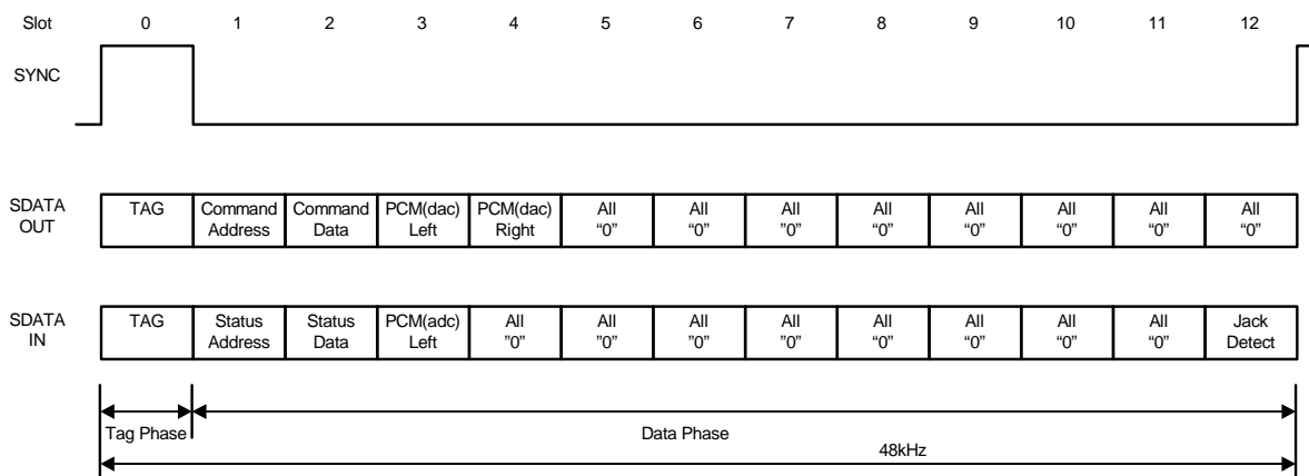
Figure 34. AC-Link protocol
