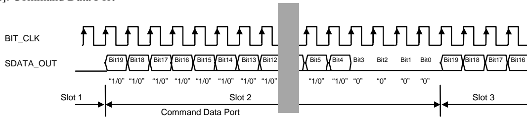
Figure 37. Slot 2
