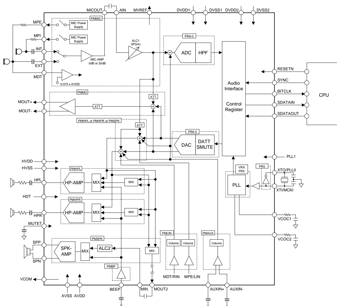
Figure 1. Block Diagram (Audio Block)
