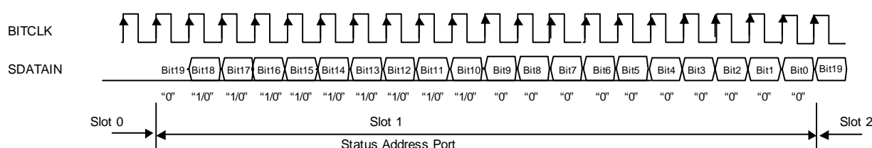
Figure 52. Slot 1
