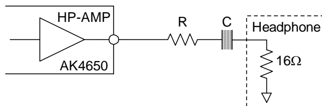
Figure 27. External Circuit Example of Headphone
