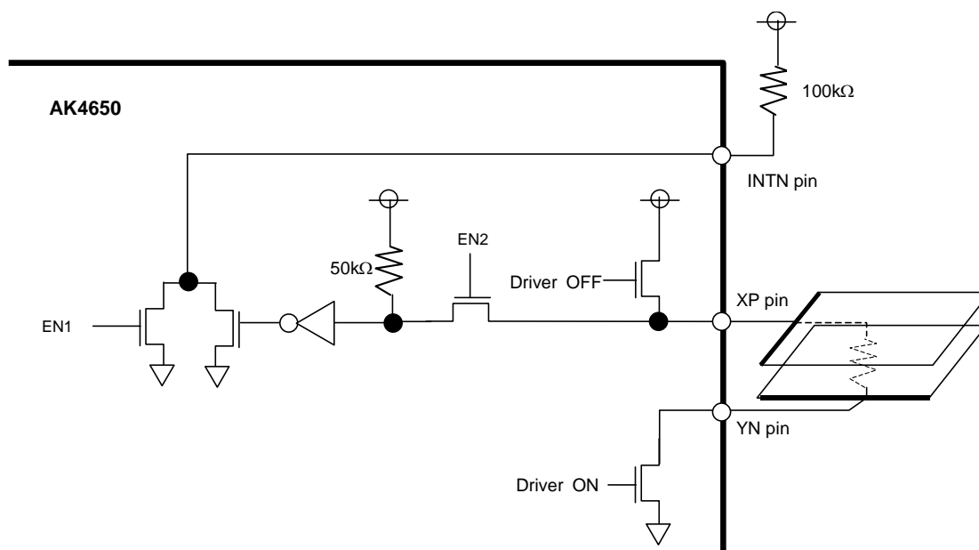
Figure 37. Pen Interrupt Block Diagram
