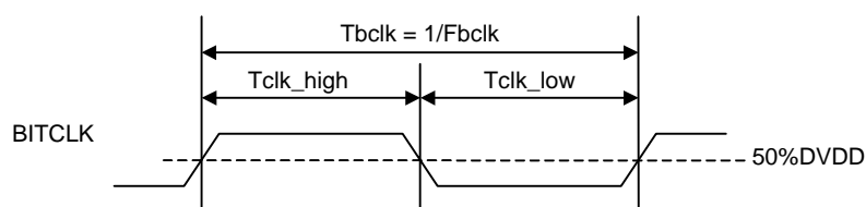
Figure 4. BITCLK Timing
