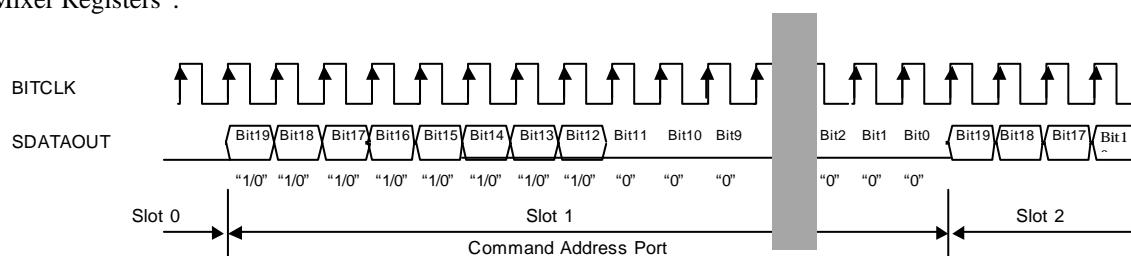
Figure 49. Slot 1
