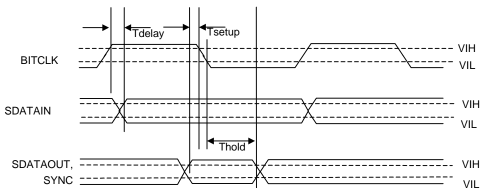
Figure 6. Setup and Hold Timing
