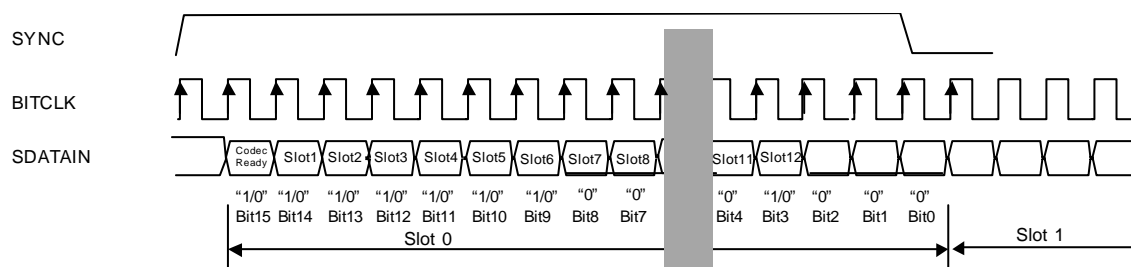
Figure 51. Slot 0
