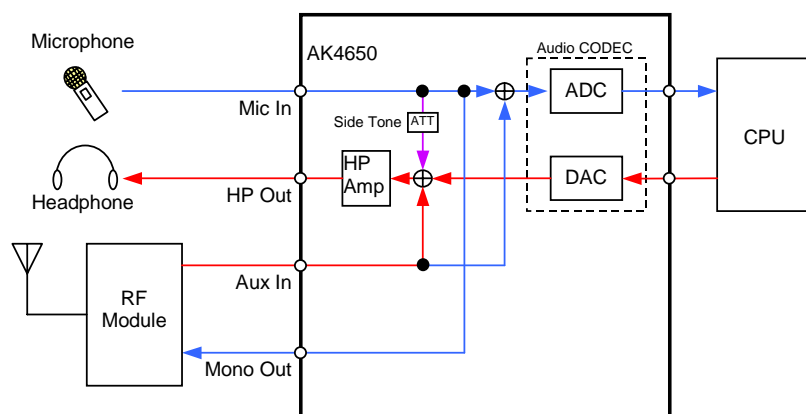
Figure 33. Recording/Playback & Phone
