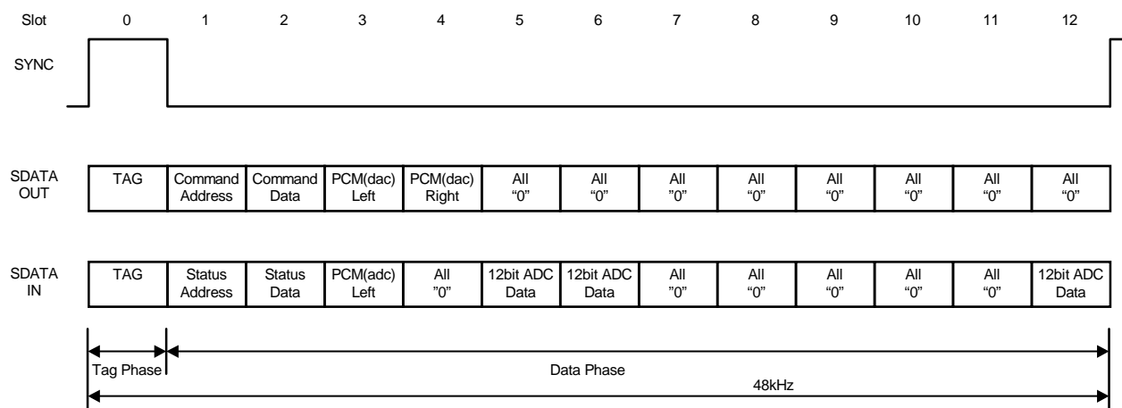
Figure 47. AC-Link protocol
