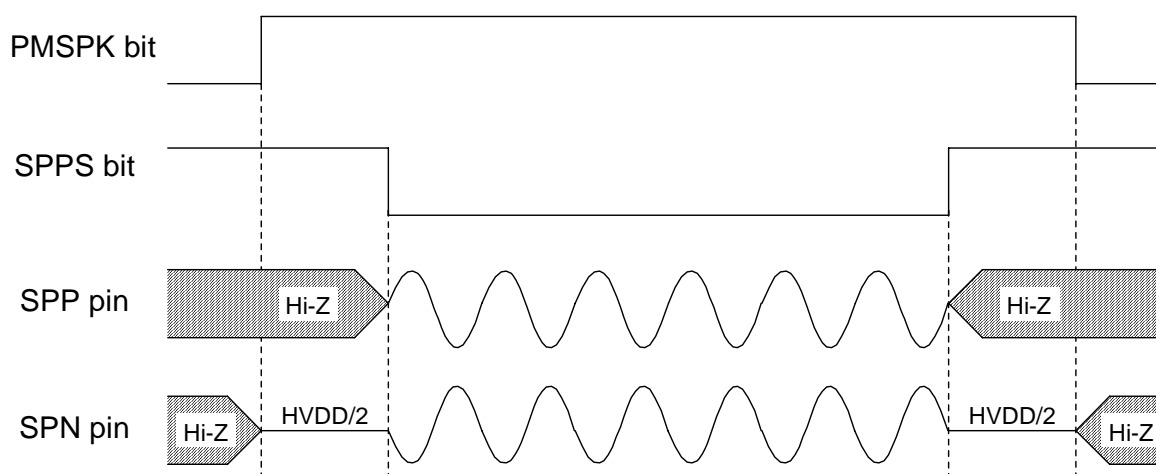
Figure 29. Power-up/Power-down Timing for Speaker-amp
