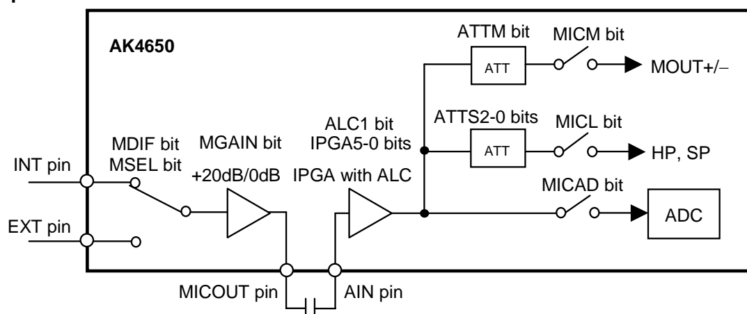
Figure 16. Microphone Input
