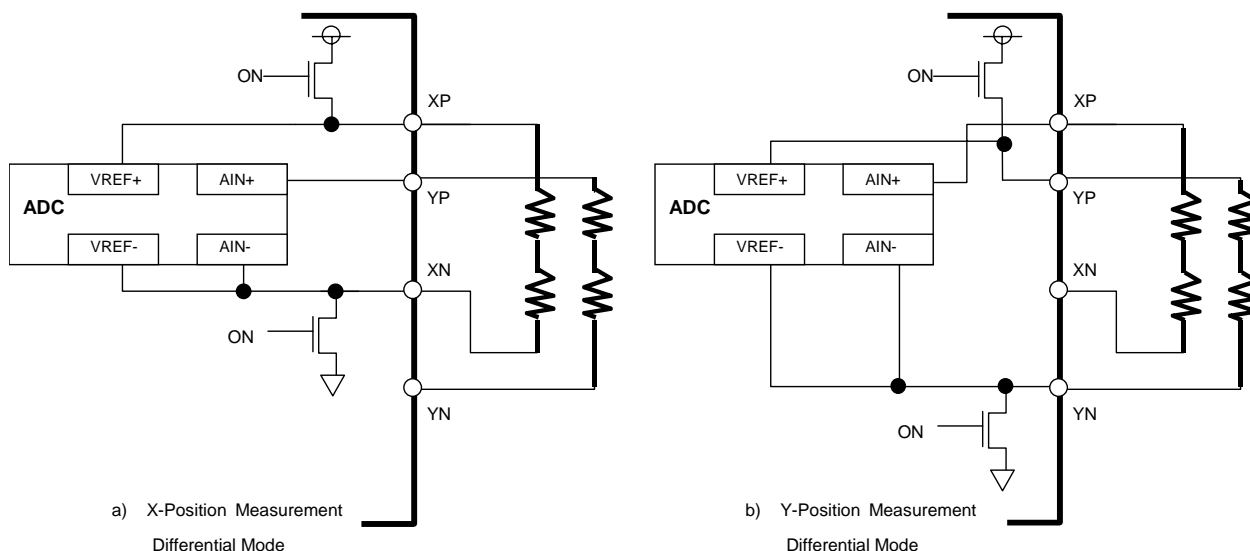
Figure 34. Axis Measurement
