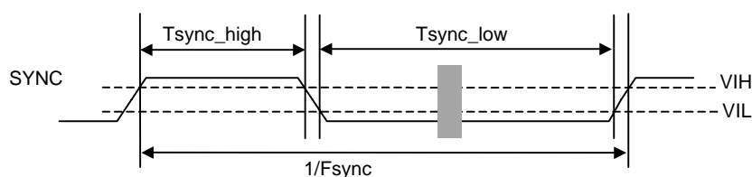
Figure 5. SYNC Timing
