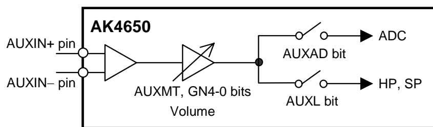
Figure 22. AUX Input
