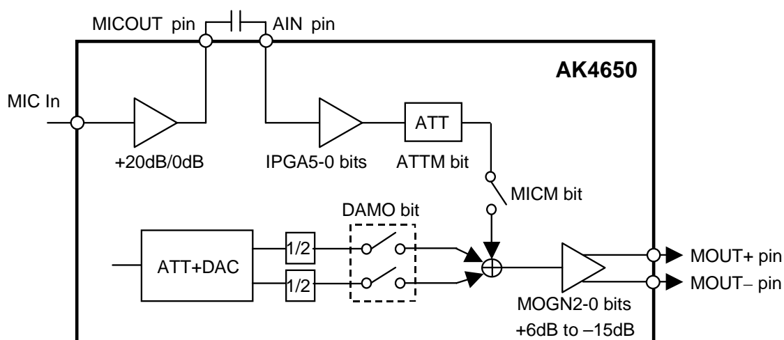
Figure 25. Mono Output
