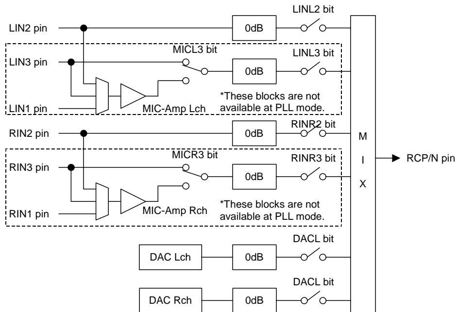
Figure 54. Receiver Mixing Circuit (AIN3 bit = "1", LOVL bit = "0")
