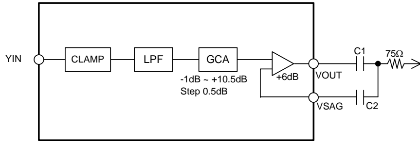
Figure 41. Video block (using Sag Compensation circuit)
