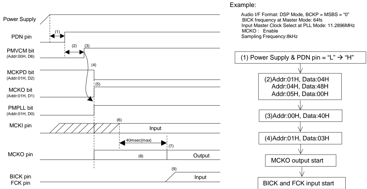
Figure 48. Clock Set Up Sequence (3)
