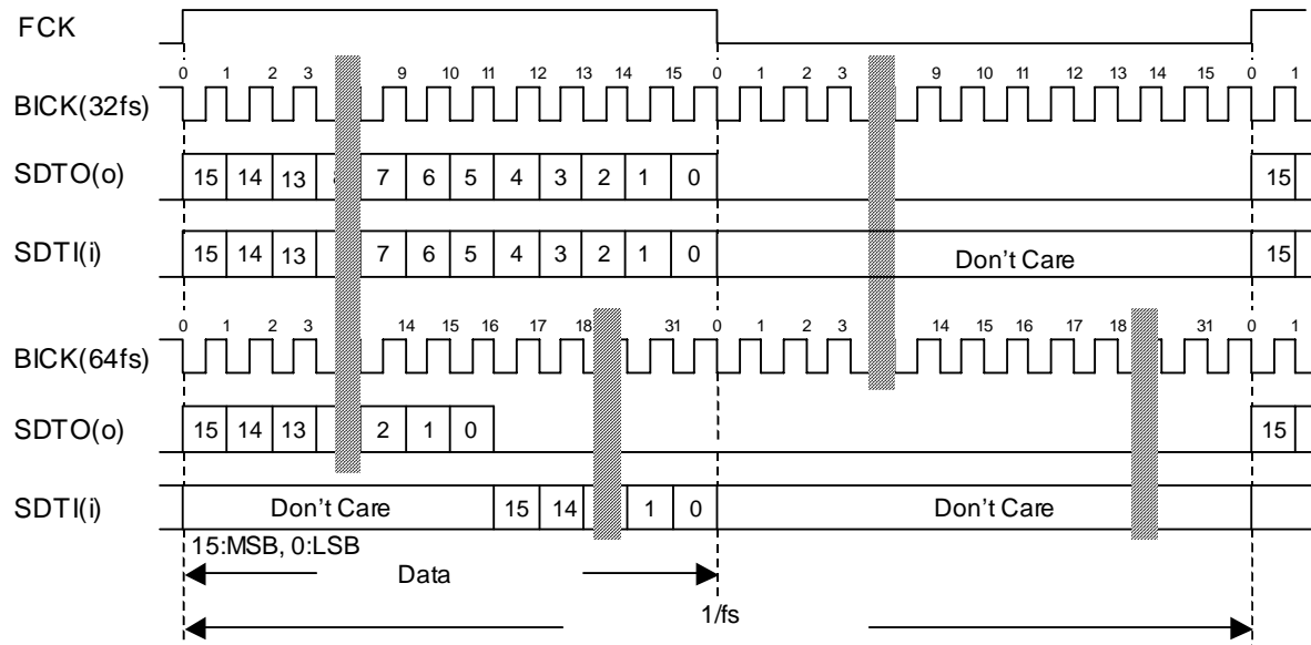
Figure 27. Mode 1 Timing
