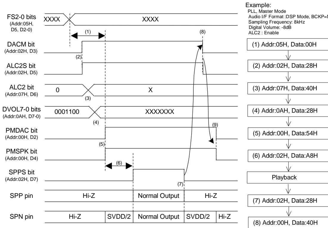
Figure 51. Speaker-Amp Output Sequence
