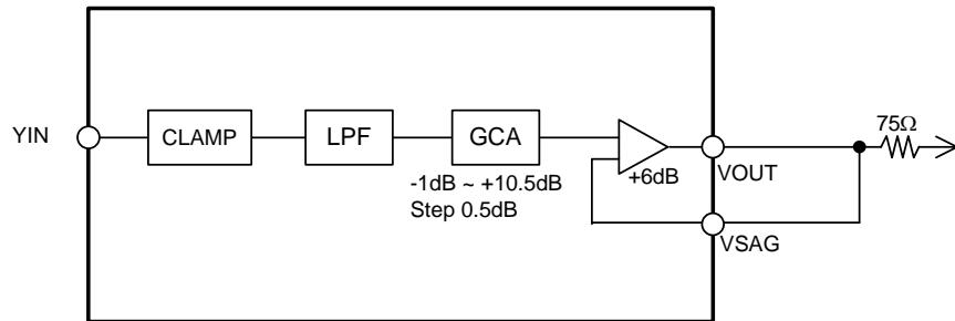
Figure 42. Video block (at DC Output)
