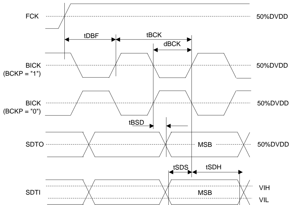
Figure 5. Audio Interface Timing (PLL Master mode &amp; DSP mode: MSBS = "1")
