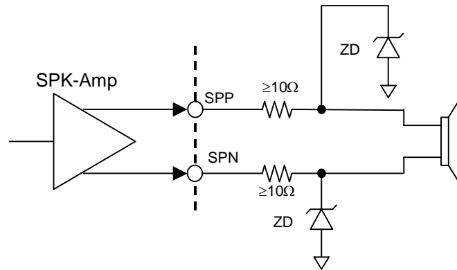
Figure 35. Circuit of Speaker Output(Load Capacitance &gt; 30pF)
