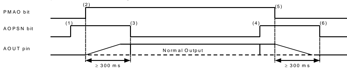
Figure 34. Mono Line Output Control Sequence in case of using POP Reduction function..
