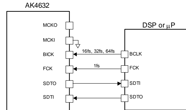
Figure 20. PLL Slave Mode 1 (PLL Reference Clock: FCK or BICK pin)
