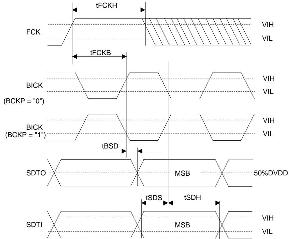
Figure 10. Audio Interface Timing (PLL Slave mode &amp; DSP mode; MSBS = 0)
