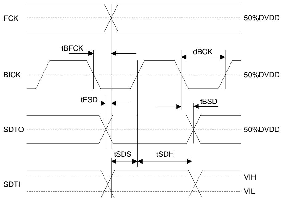
Figure 6. Audio Interface Timing (PLL Master mode &amp; Except DSP mode)
