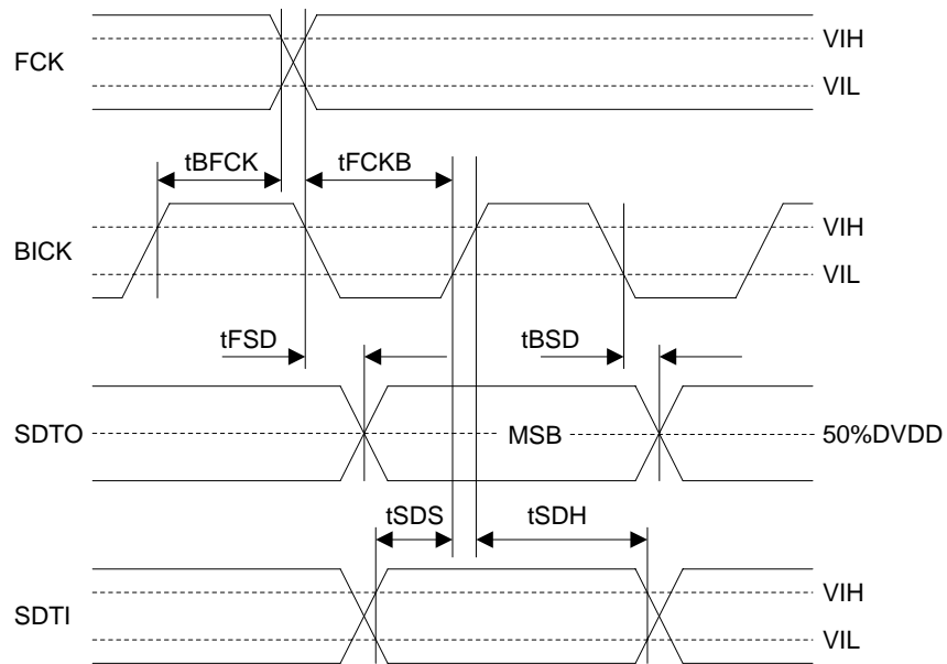
Figure 13. Audio Interface Timing (PLL, EXT Slave mode &amp; Except DSP mode)
