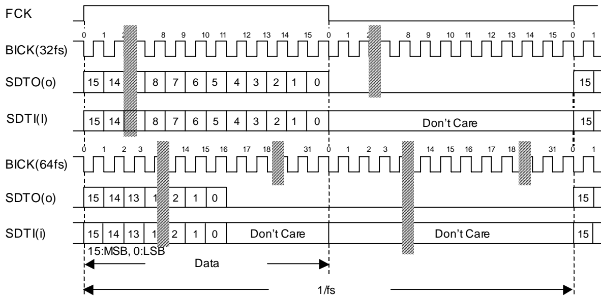
Figure 28. Mode 2 Timing
