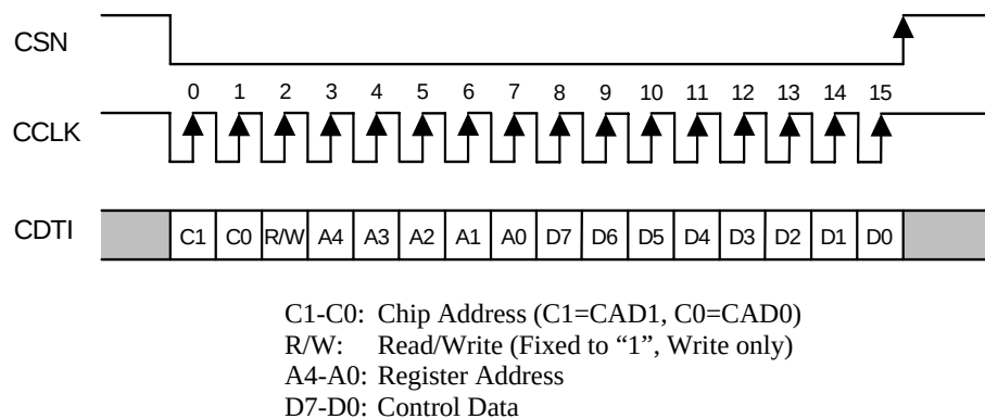
Figure 17. 3-wire Serial Control I/F Timing
