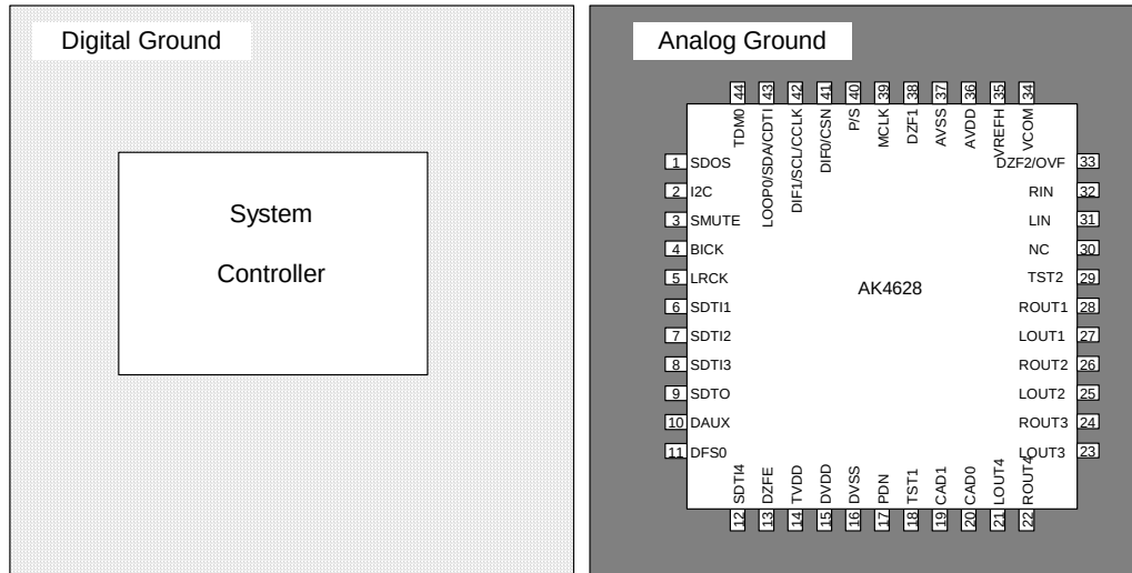
Figure 26. Ground Layout
