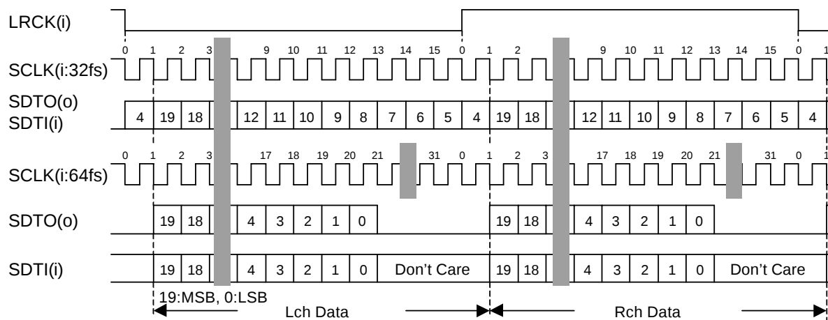
Figure 5. Mode 3 Timing
