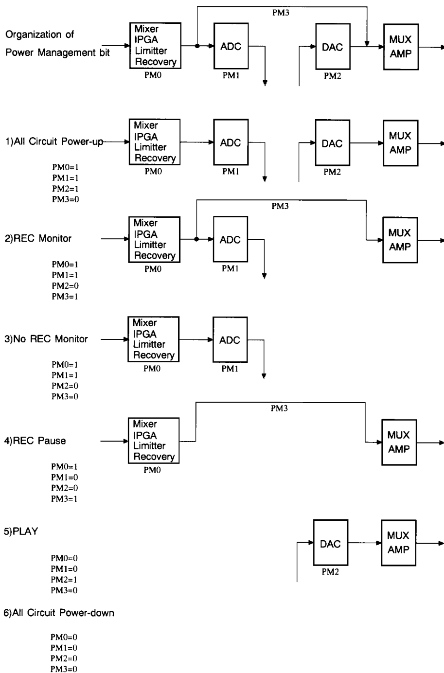
Figure 11. Power Management
