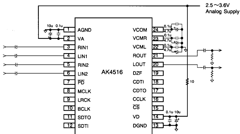
Figure 13. Typical Connection Diagram
