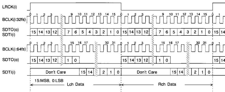
Figure 1. Audio Data Timing (No.0)
