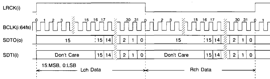
Figure 2. Audio Data Timing (No.1)
