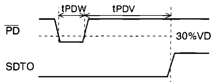
Reset Timing
