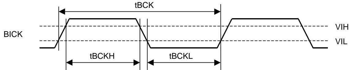
Clock Timing
