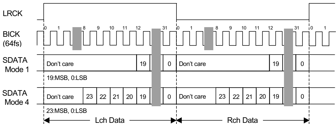
Figure 2. Mode 1,4 Timing
