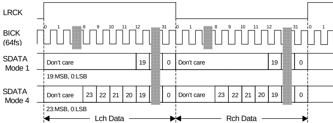
Figure 2. Mode 1,4 Timing
