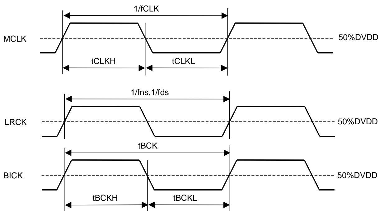
Clock Timing
