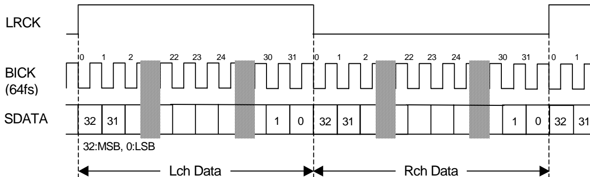
Figure 5. Mode 5/6 Timing
