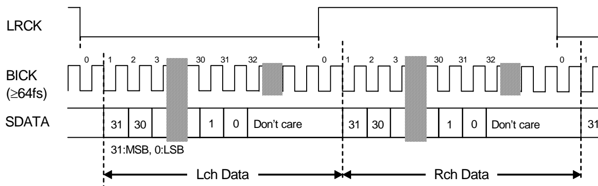
Figure 6. Mode 7 Timing
