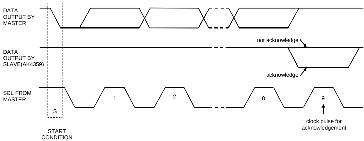
Figure 20. Acknowledge on the I²C-bus
