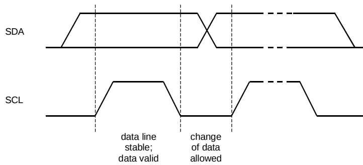
Figure 21. Bit transfer on the I²C-bus
