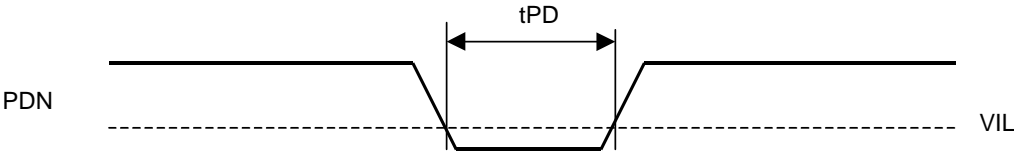
Power-down Timing
