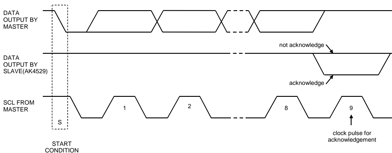
Figure 23. Acknowledge on the I 2 C-bus
