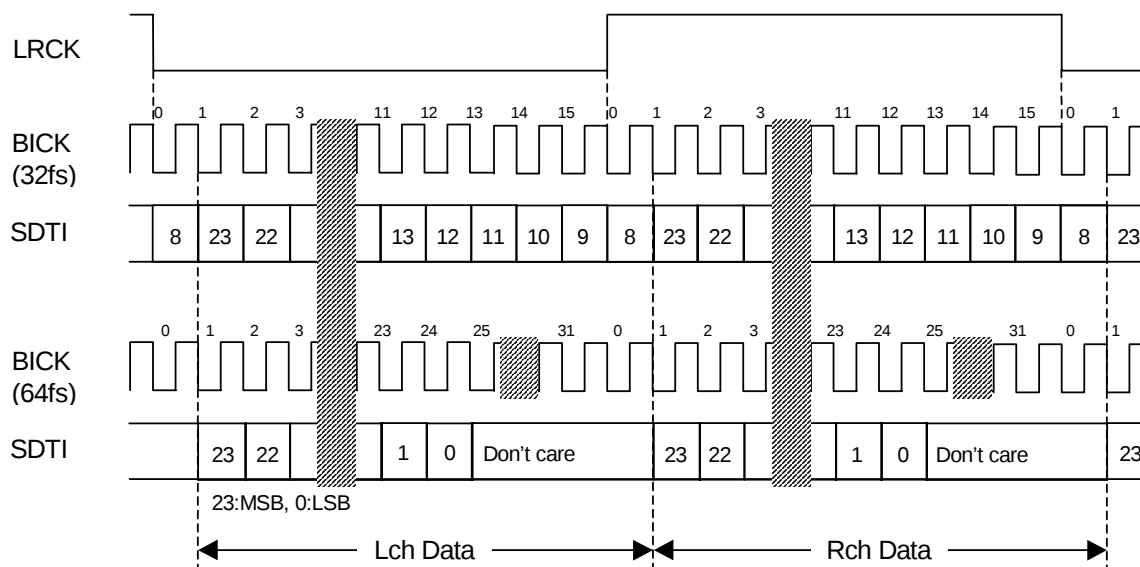
Figure 4. Mode 3 Timing
