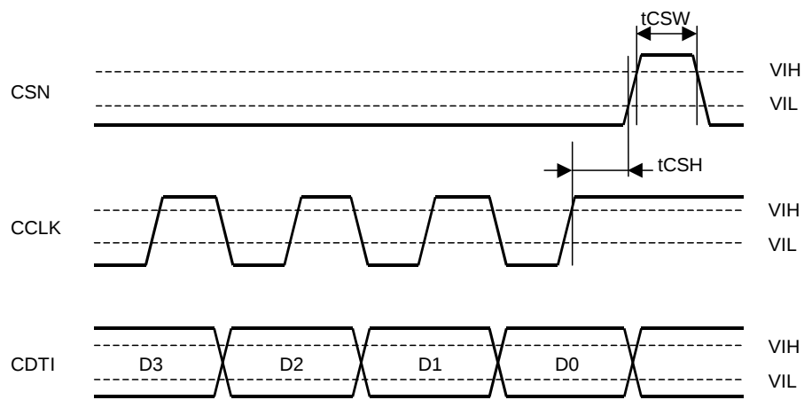
WRITE Data Input Timing
