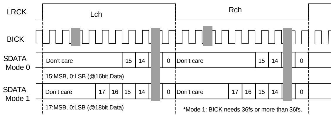
Figure 2. Mode 0,1 Timing
