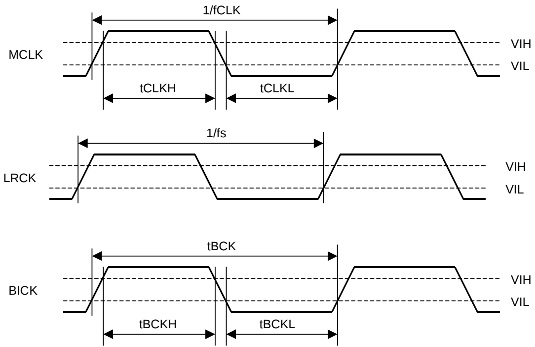
Clock Timing
