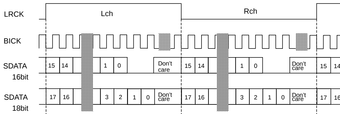
Figure 2. Mode 2 Timing
