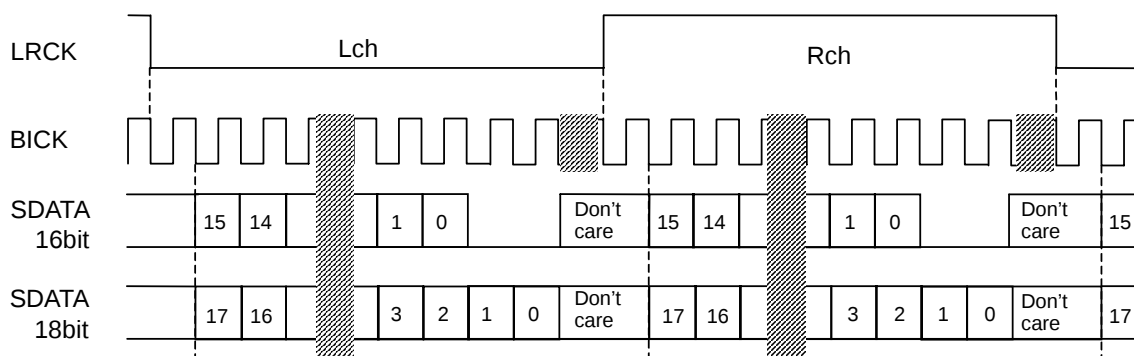
Figure 3. Mode 3 Timing
