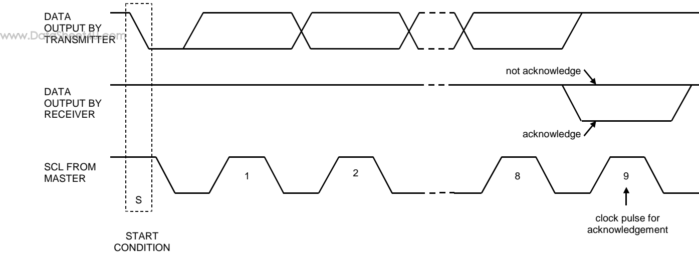
Figure 13. Acknowledge on the I 2 C-Bus
