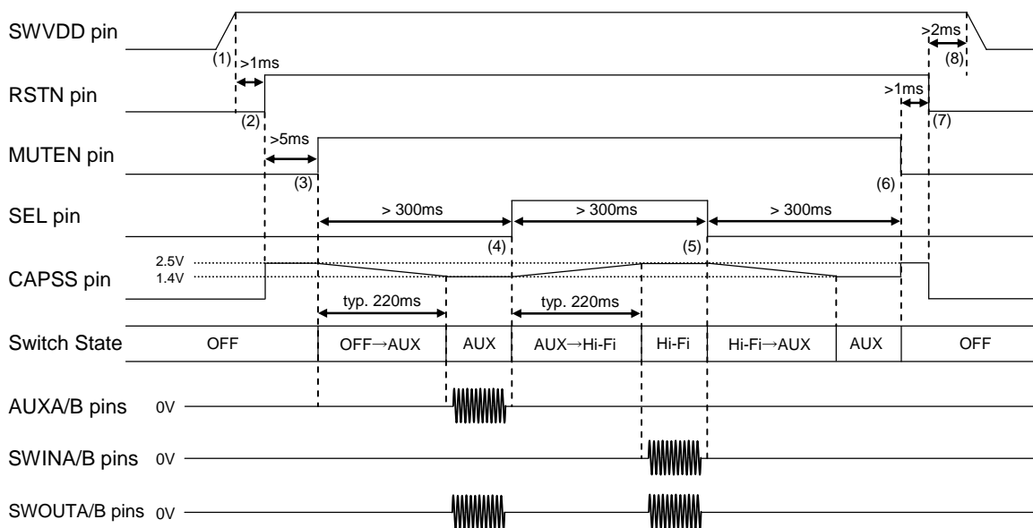
Figure 13. Power-Up/Down Sequence
