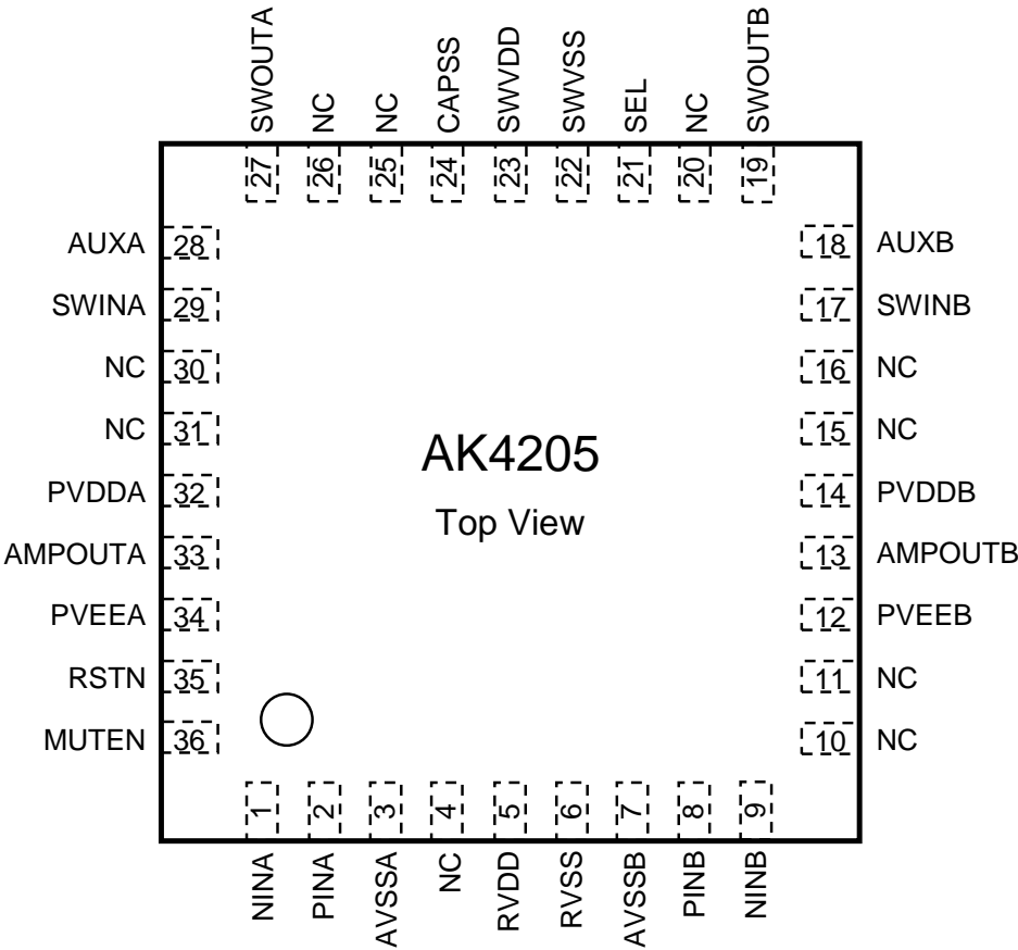
Figure 2. Pin Configurations
