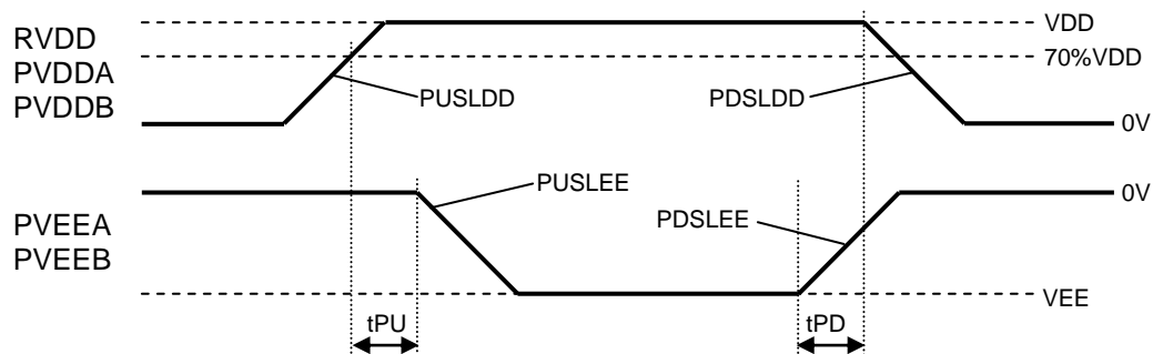
Figure 9. Headphone-amp Power-up/down Timing
