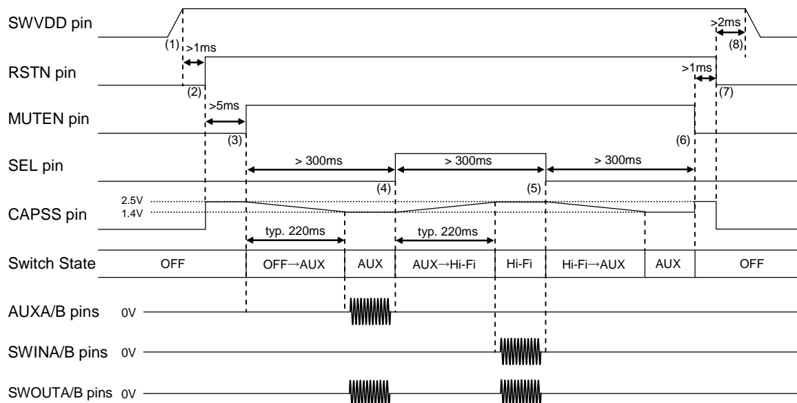
Figure 13. Power-Up/Down Sequence
