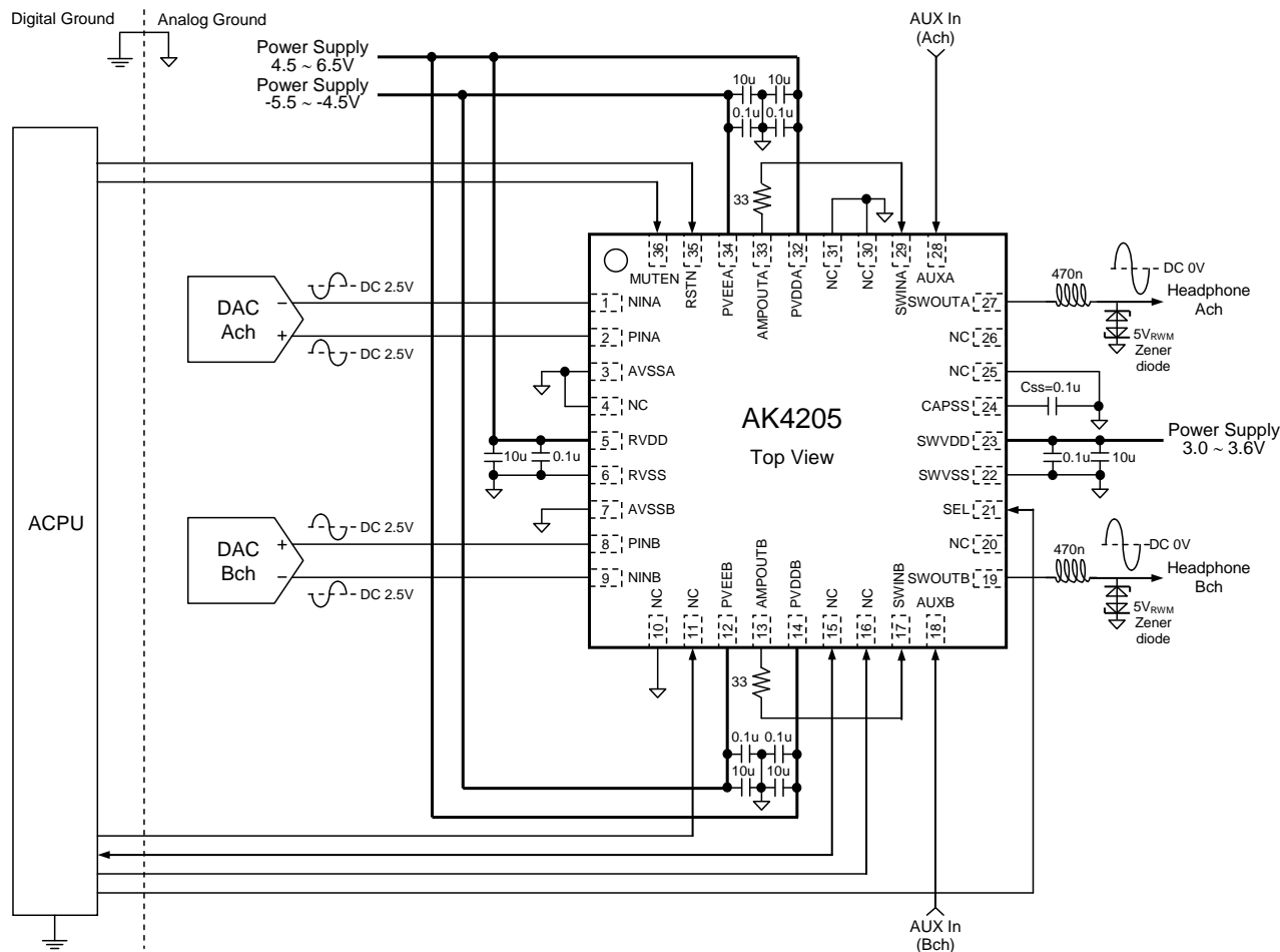
Figure 15. Circuit Example with AK4205
