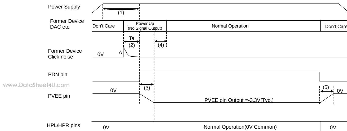
Figure 4. Power-up/down Sequence example
