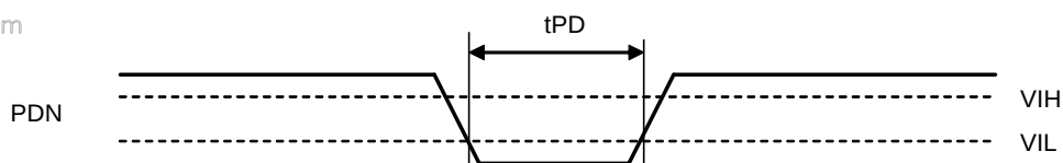
Figure 2. Power-down Timing
