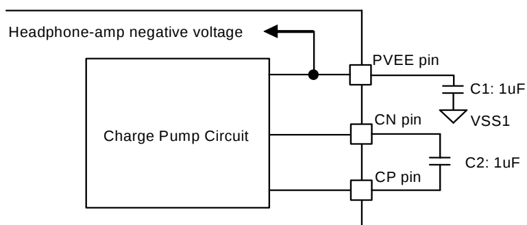
Figure 3. Charge Pump Circuit External Capacitor
