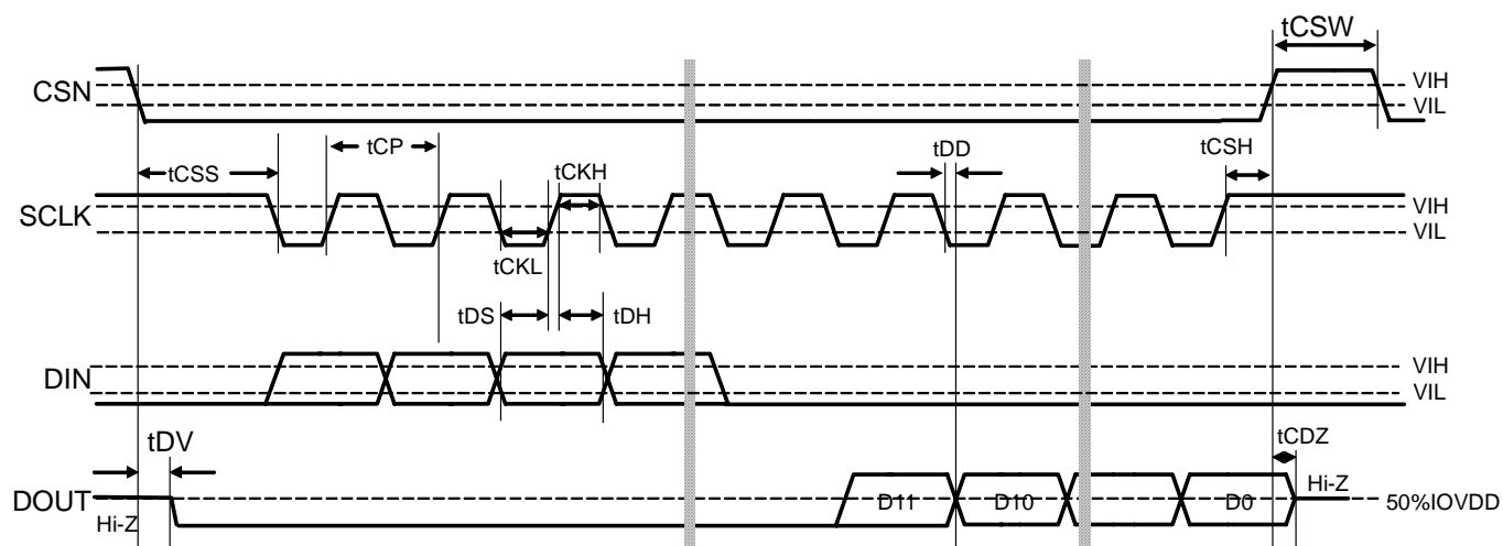
Figure 1. Timing Diagram
