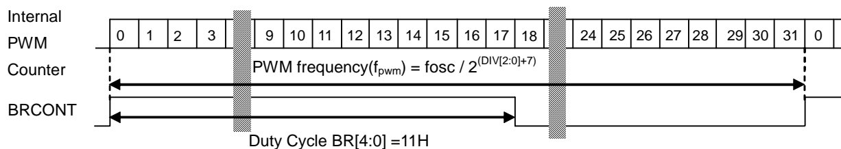
Figure 16. PWM output waveform
