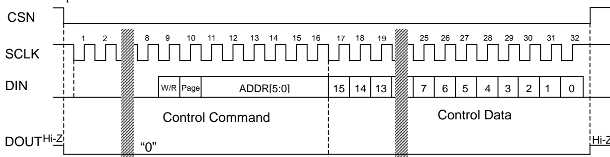
Figure 10. Write Operation
