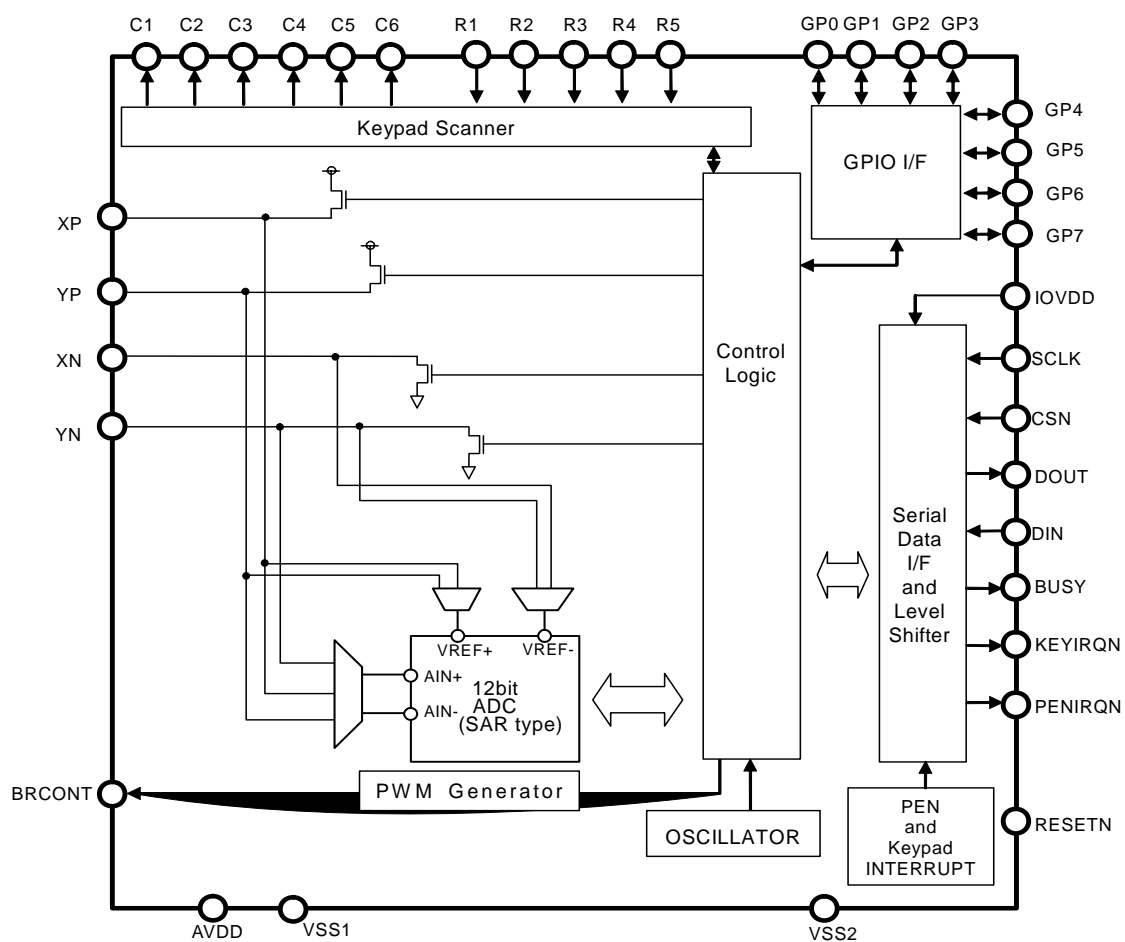
Block Diagram
