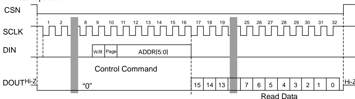
Figure 11. Read Operation
