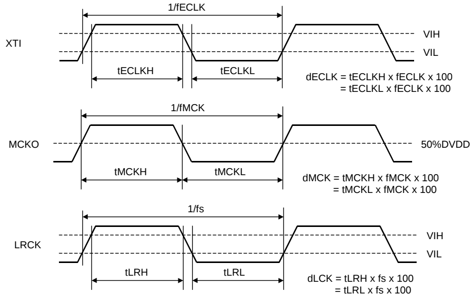
Figure 1. Clock Timing
