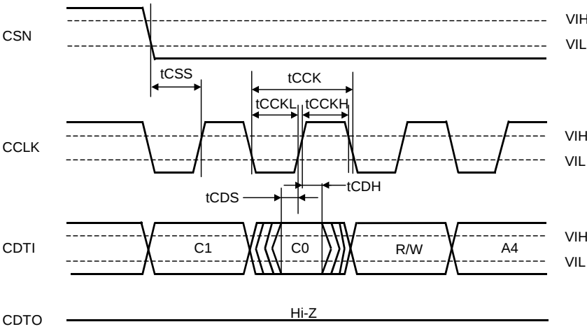
Figure 3. WRITE/READ Command Input Timing
