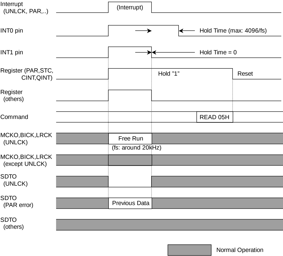
Figure 16. INT1-0 pin timing
