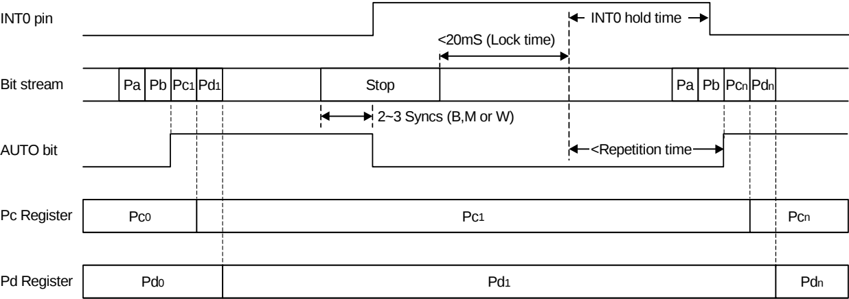
Figure 27. Timing example 2
