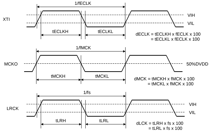
Figure 1. Clock Timing
