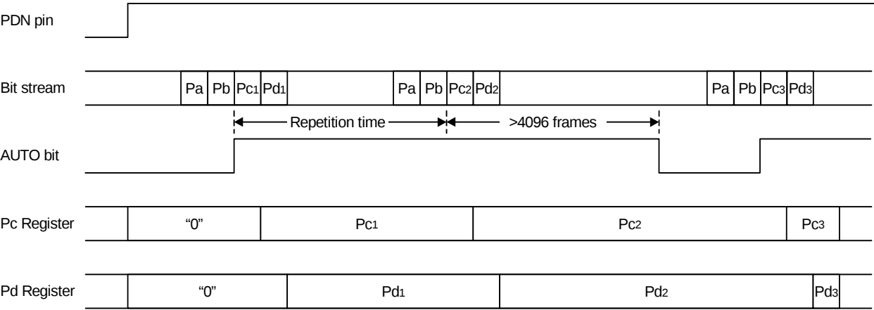
Figure 26. Timing example 1
