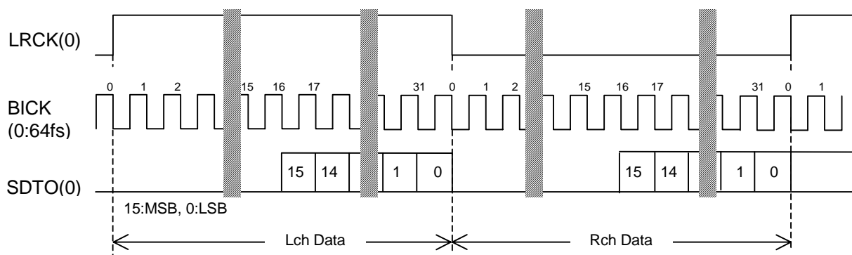
Figure 35. Mode 0 Timing
