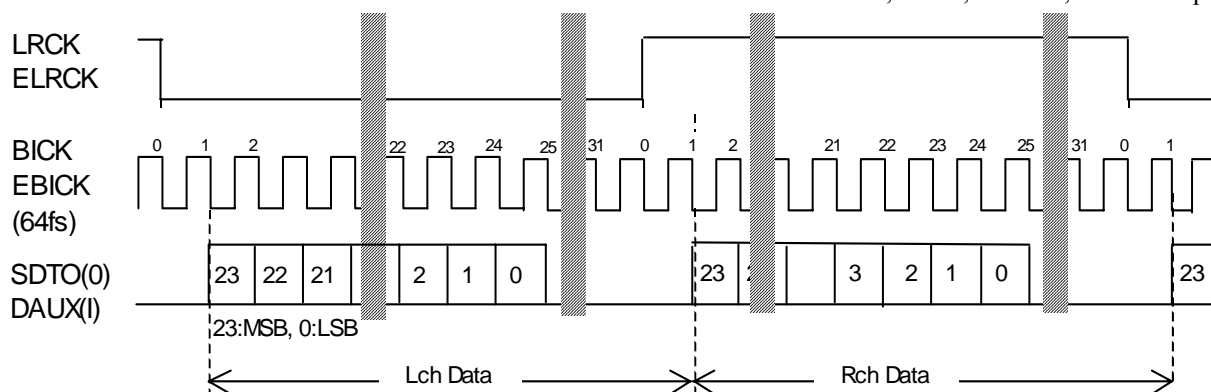
Figure 38. Mode 5, 7 Timing
