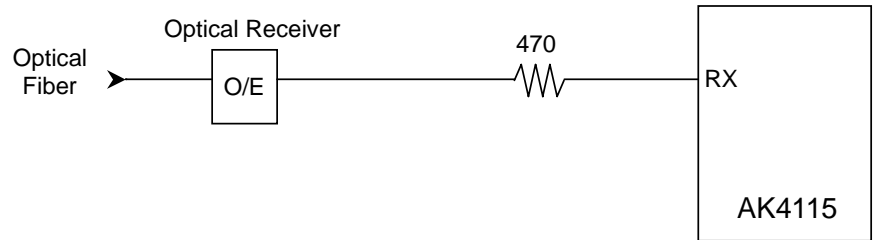
Figure 22. Consumer Input Circuit (Optical Input)
