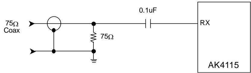
Figure 21. Consumer Input Circuit (Coaxial Input)
