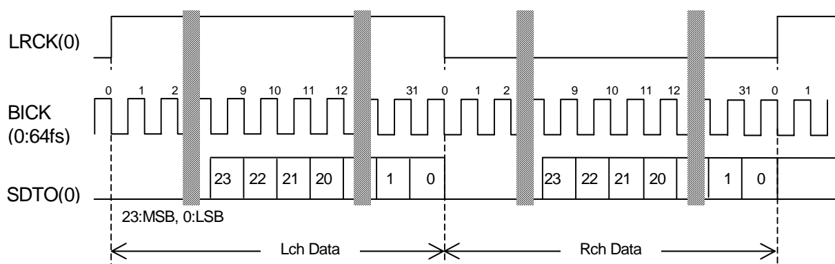
Figure 36. Mode 3 Timing
