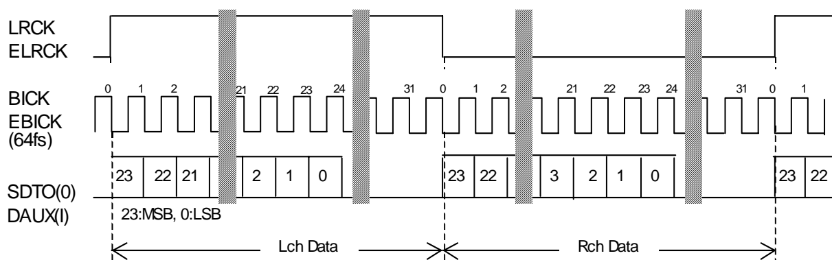
Figure 37. Mode 4, 6 Timing
